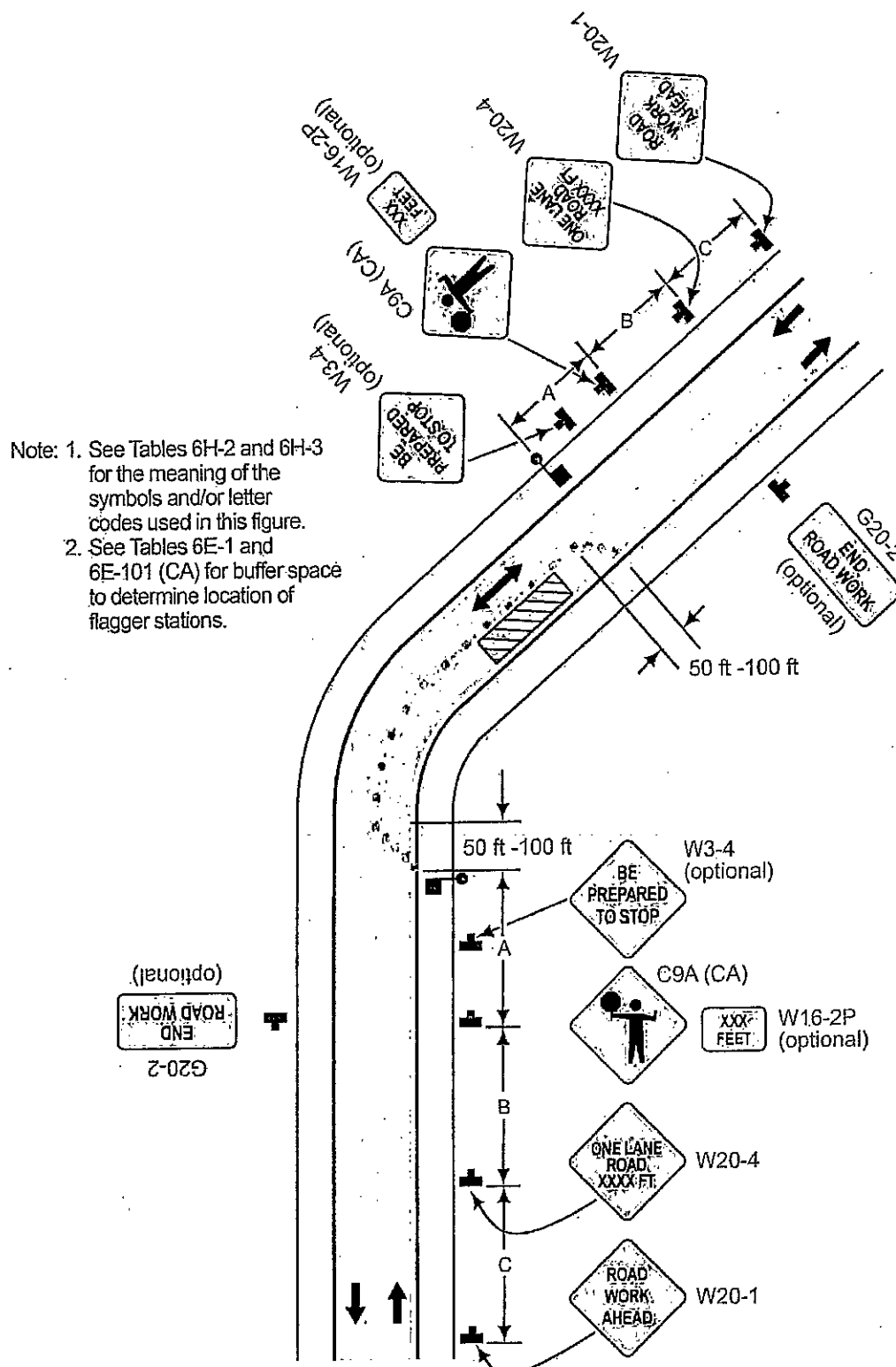
Typical Application 10
