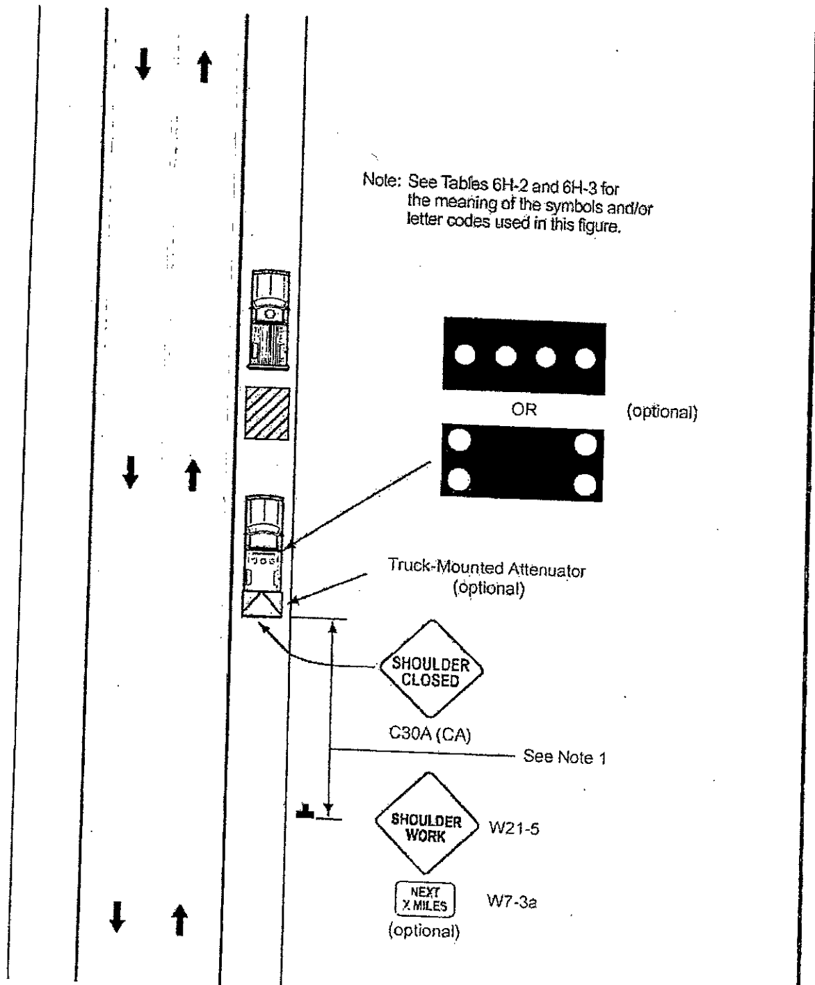
Typical Application 4
