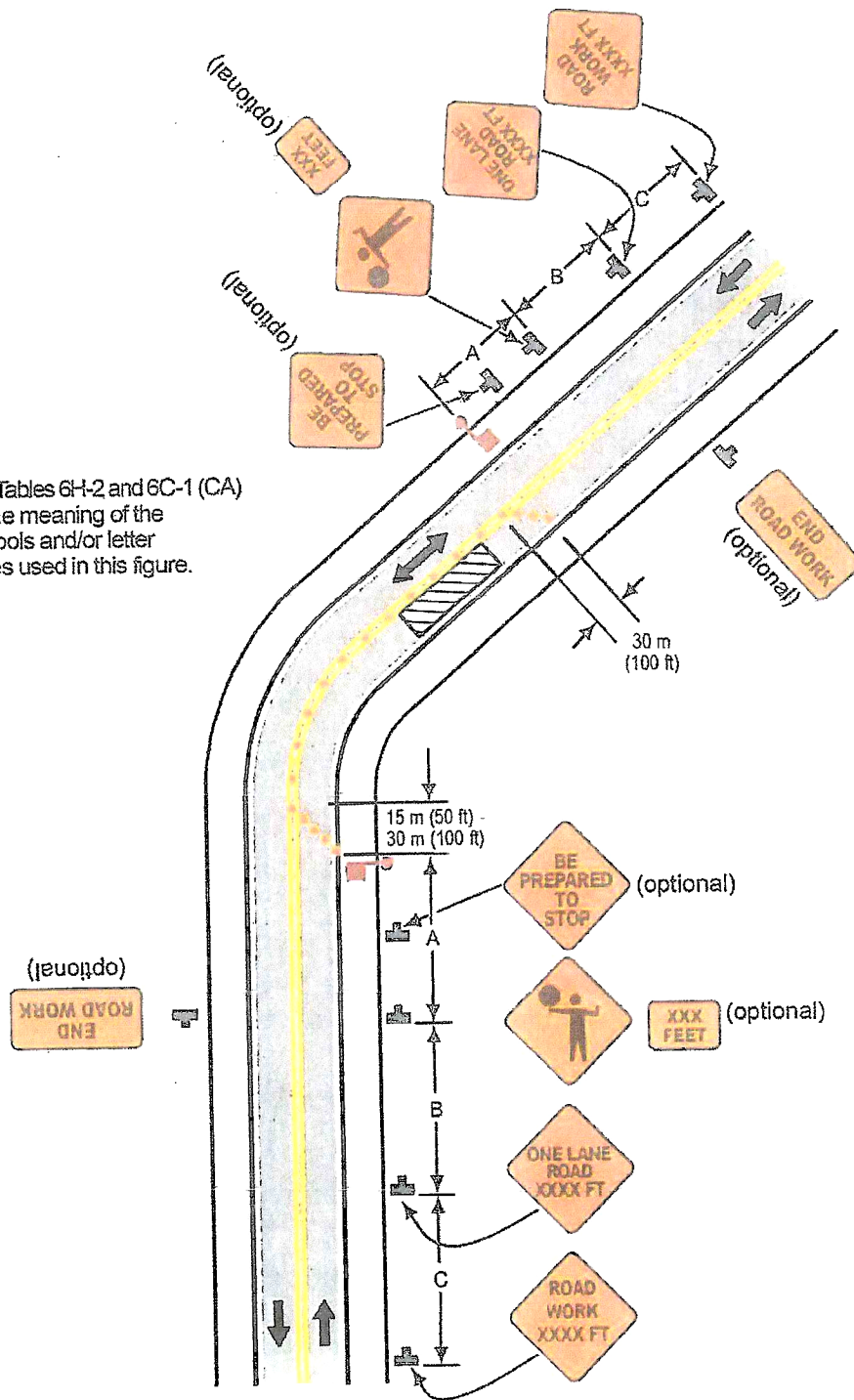
Typical Application 10
