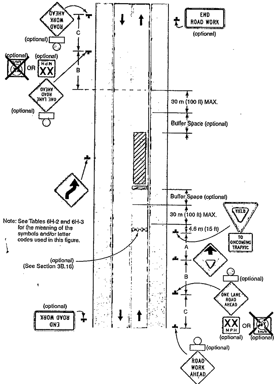
Typical Application 11
