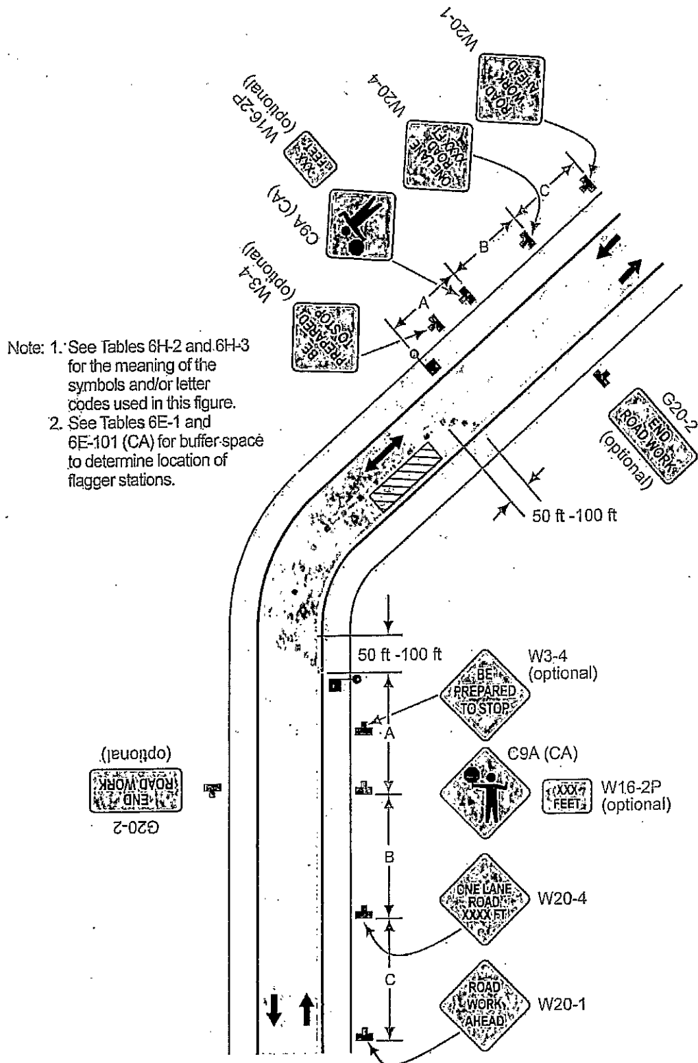
Typical Application 10
