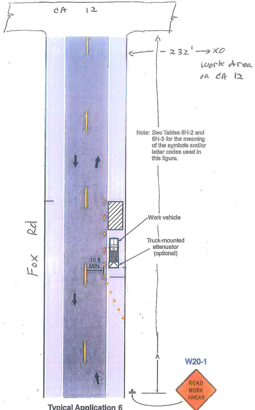
Figure 6H-6. Shoulder Work with Minor Encroachment (TA-6)
