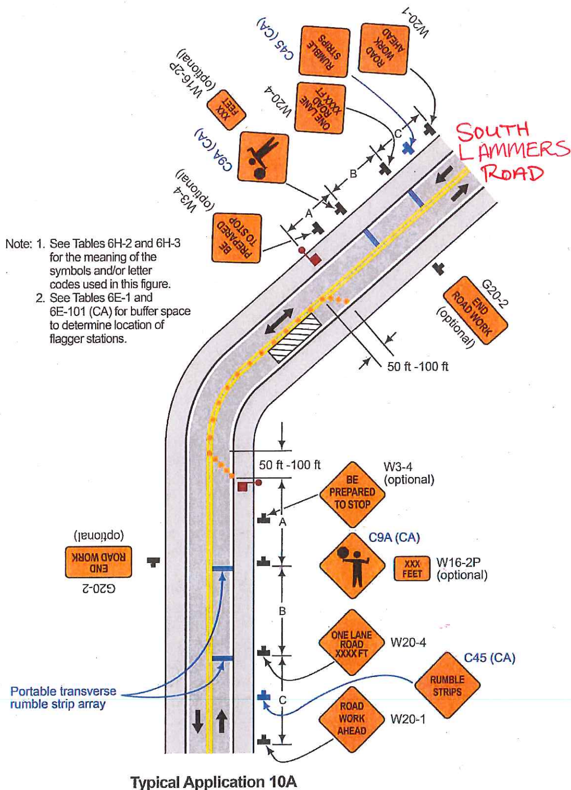
Figure 6H-10A (CA). Lane Closure on Two-Lane Road Using Flaggers (TA-10A) Using Portable Transverse Rumble Strips
