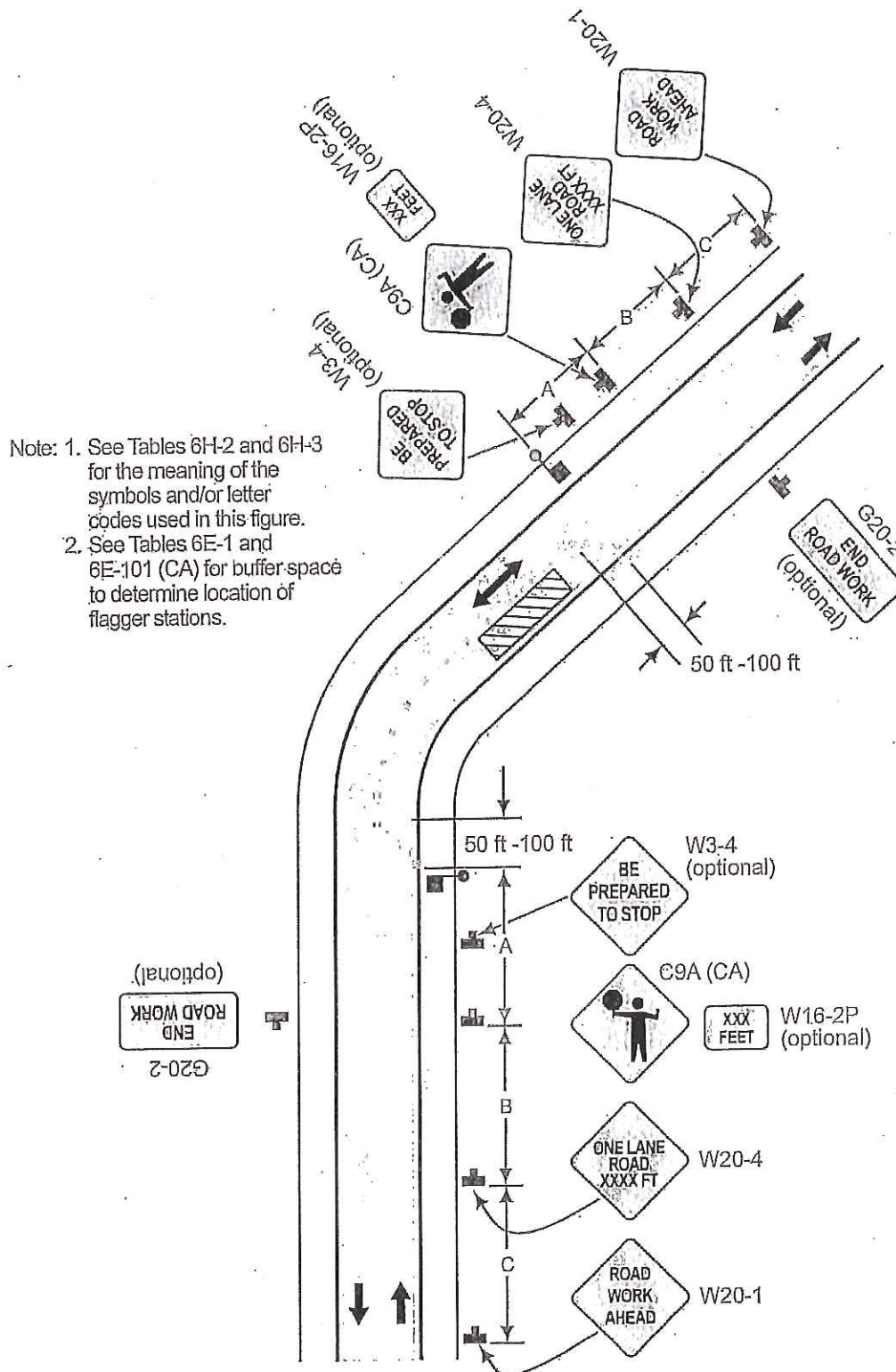
Typical Application 10
