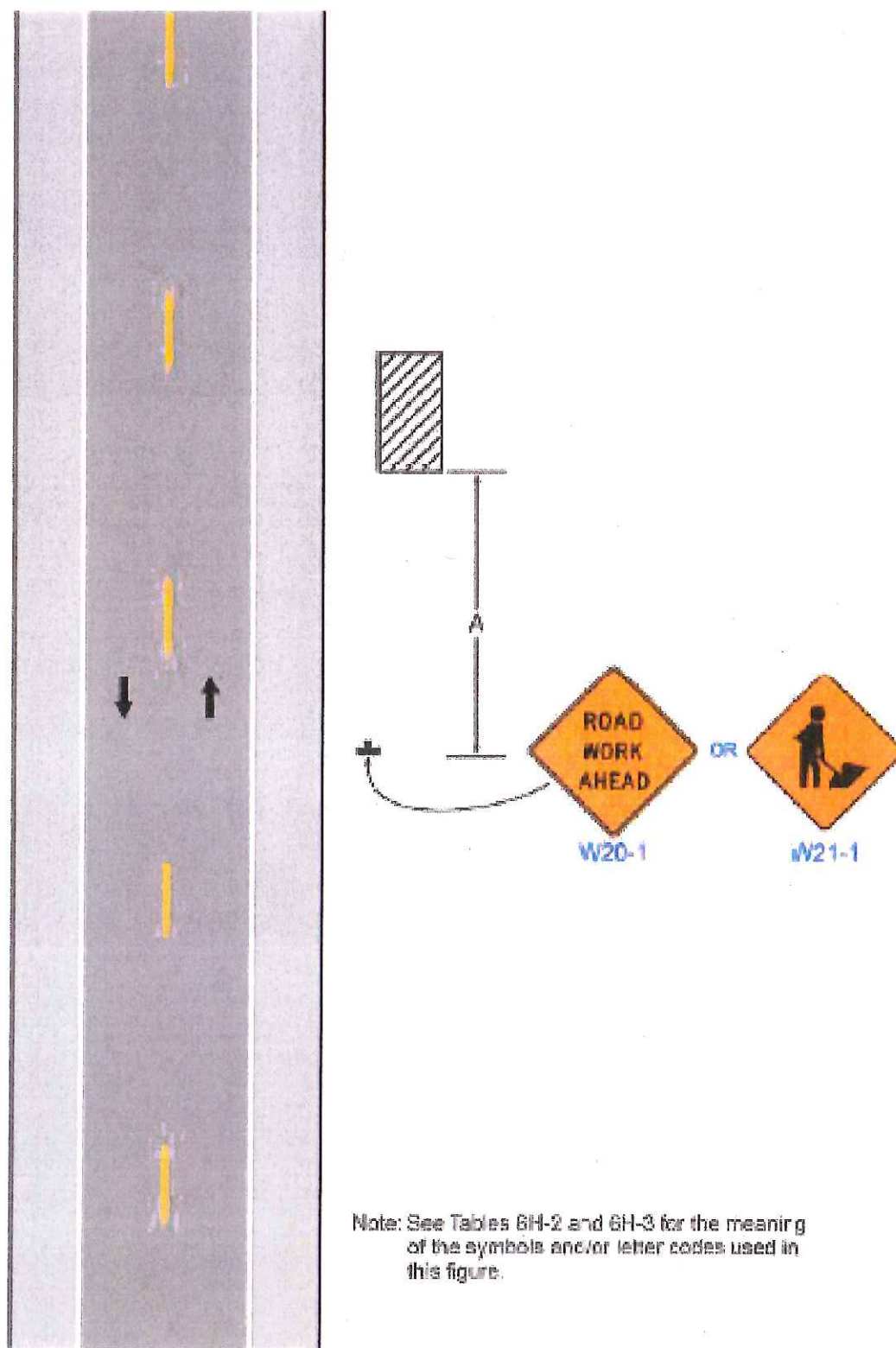
Typical Application 1
