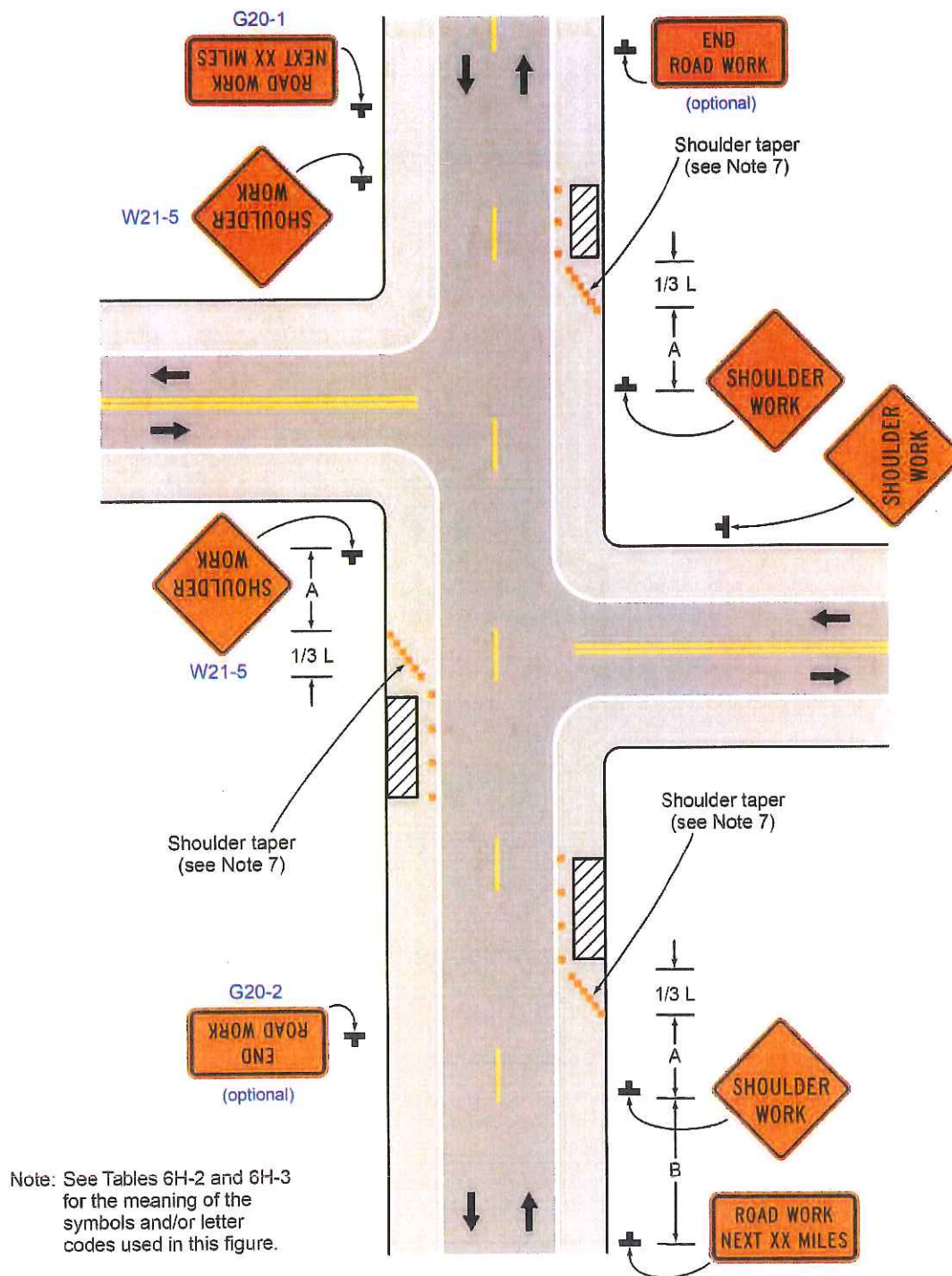
Typical Application 3
