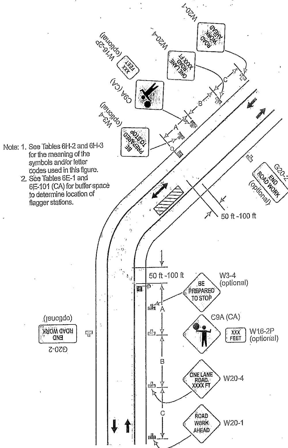
Typical Application 10
