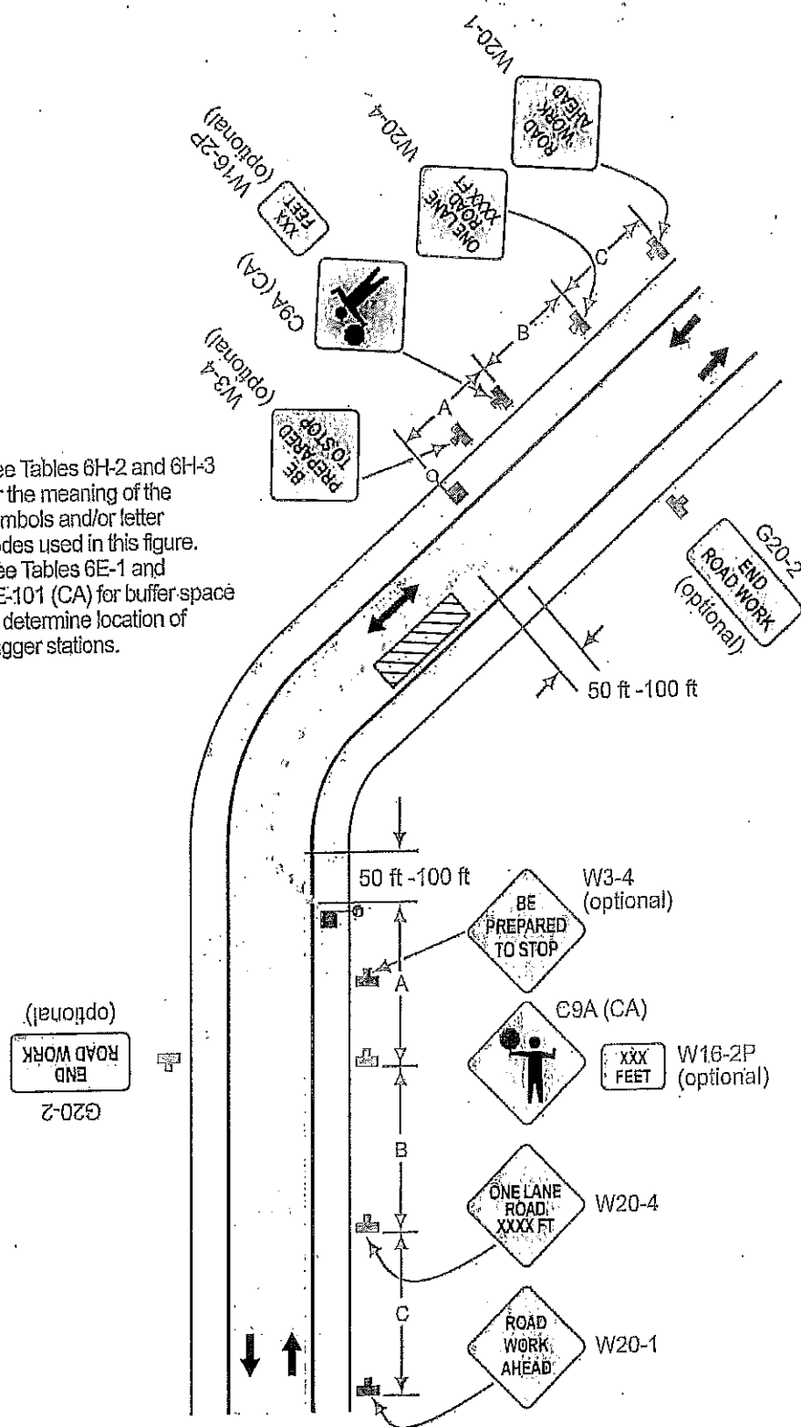
Typical Application 10
