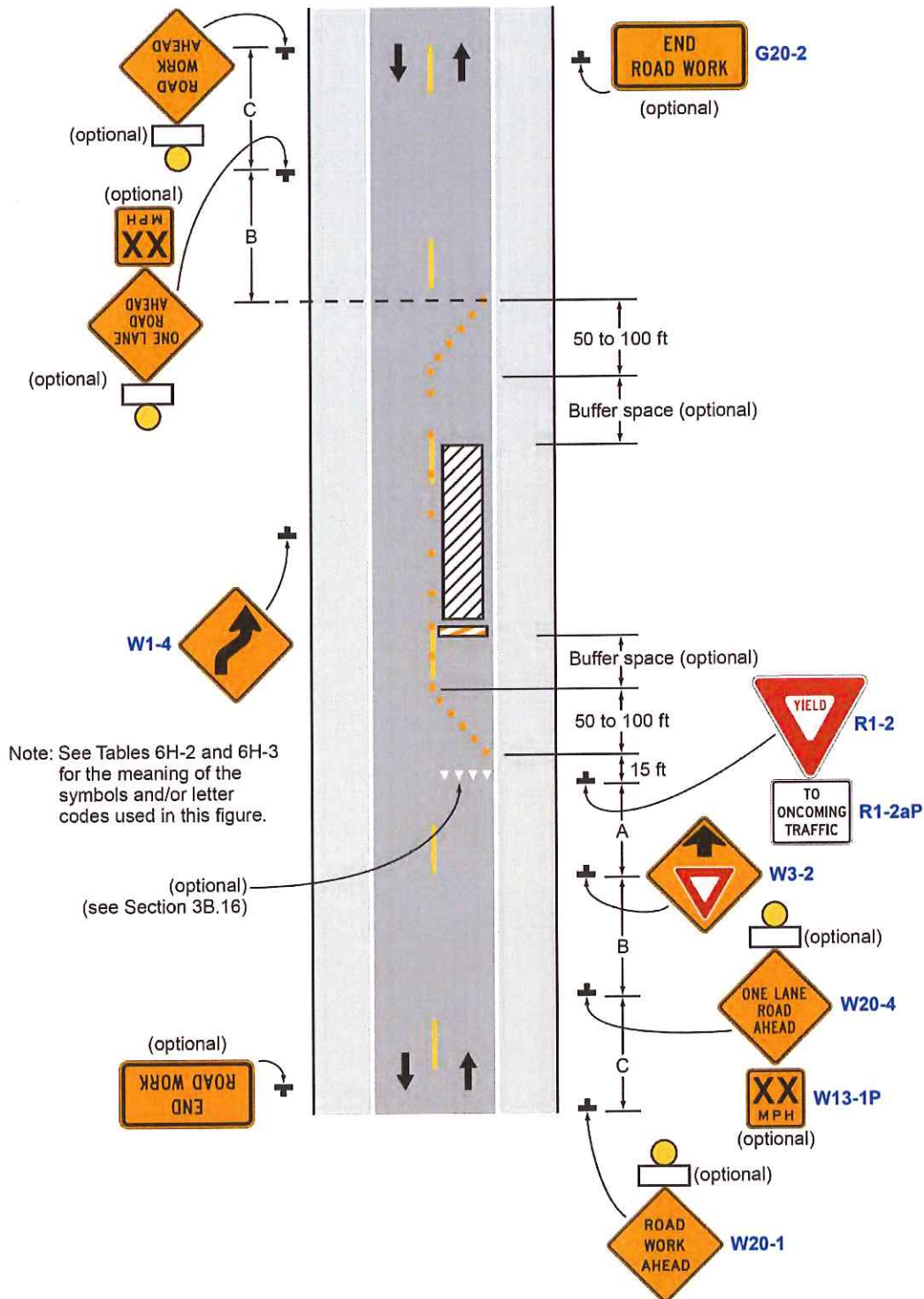
Typical Application 11
