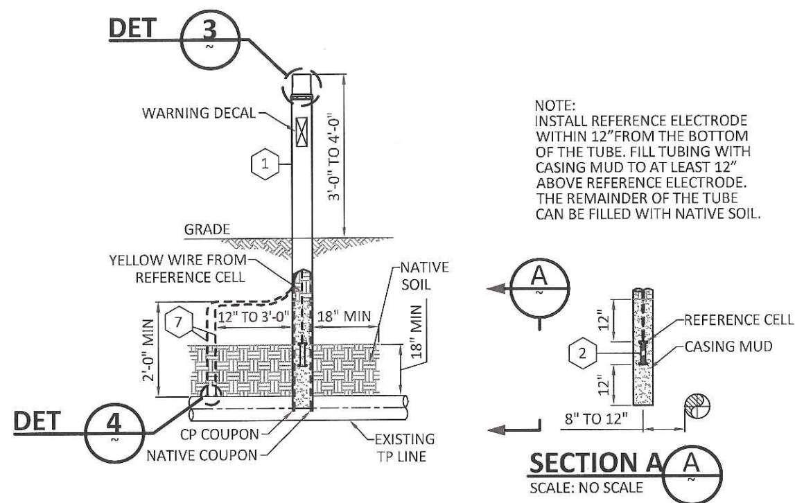
DETAIL 1 SCALE: NO SCALE COUPON TEST STATION ABOVE GROUND SHTS 10-23 CCV O-10.2
