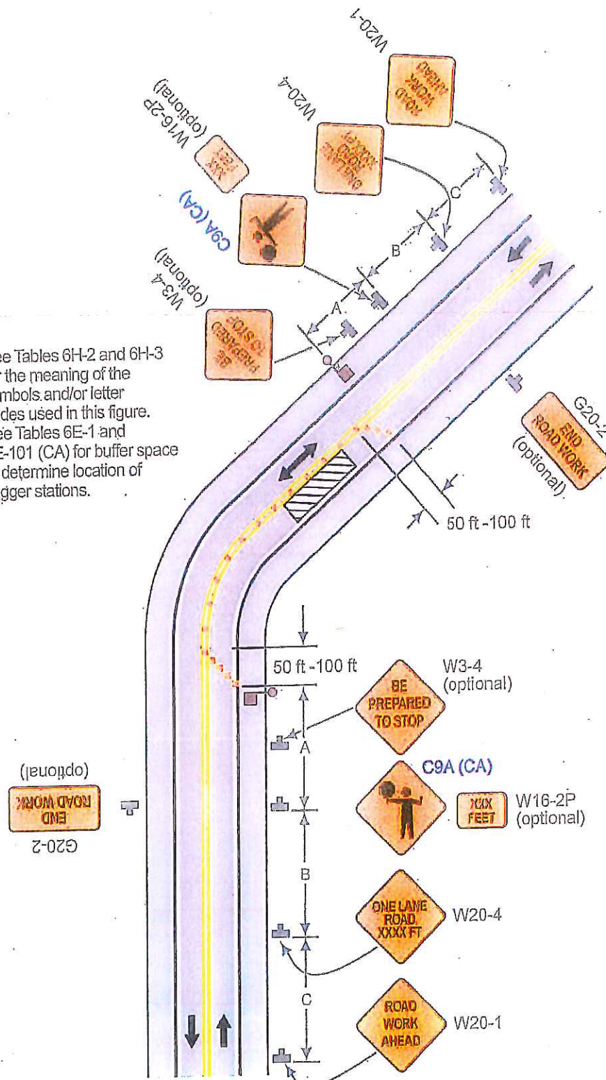
Typical Application 10
