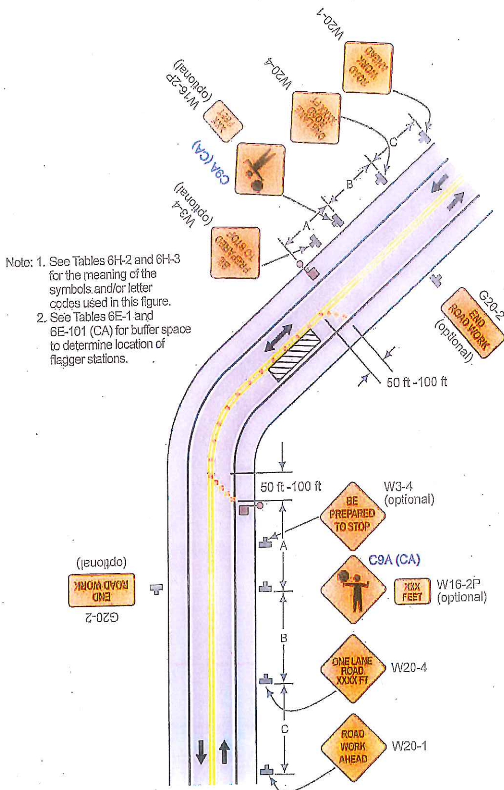
Typical Application 10
