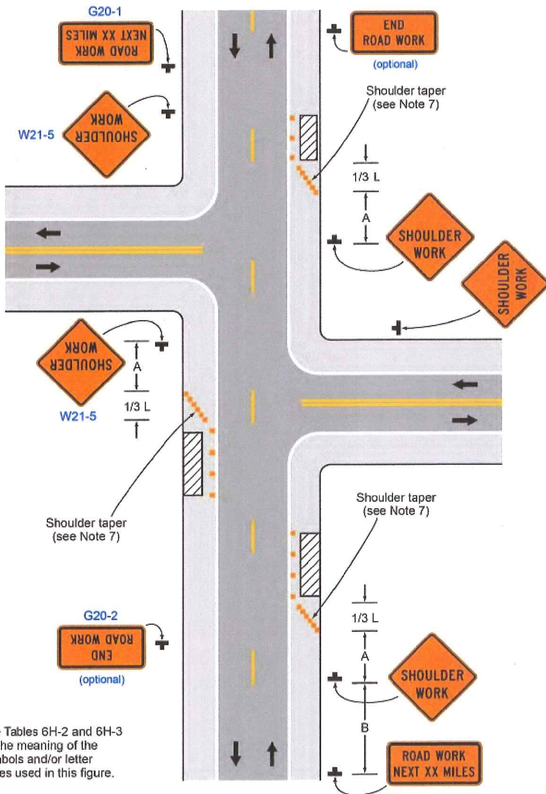
Typical Application 3
