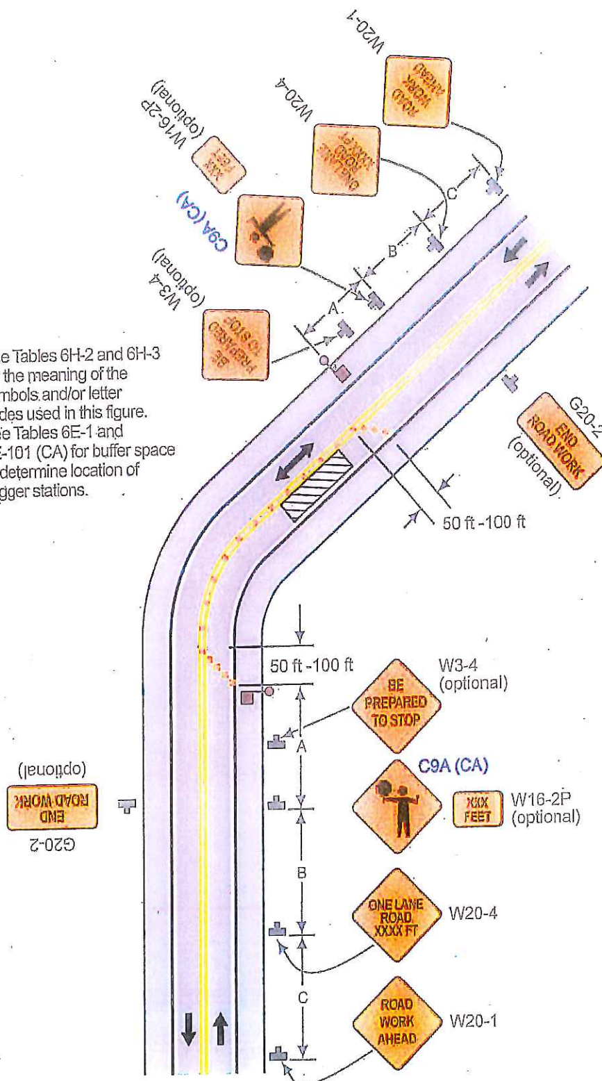
Typical Application 10
