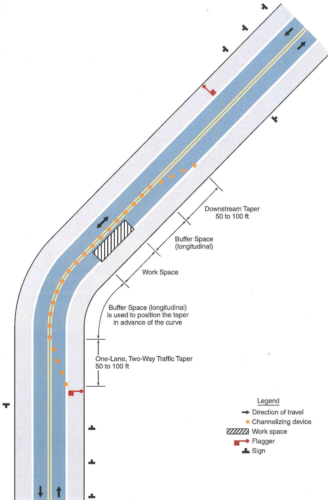
Figure 6C-3. Example of a One-Lane, Two-Way Traffic Taper
