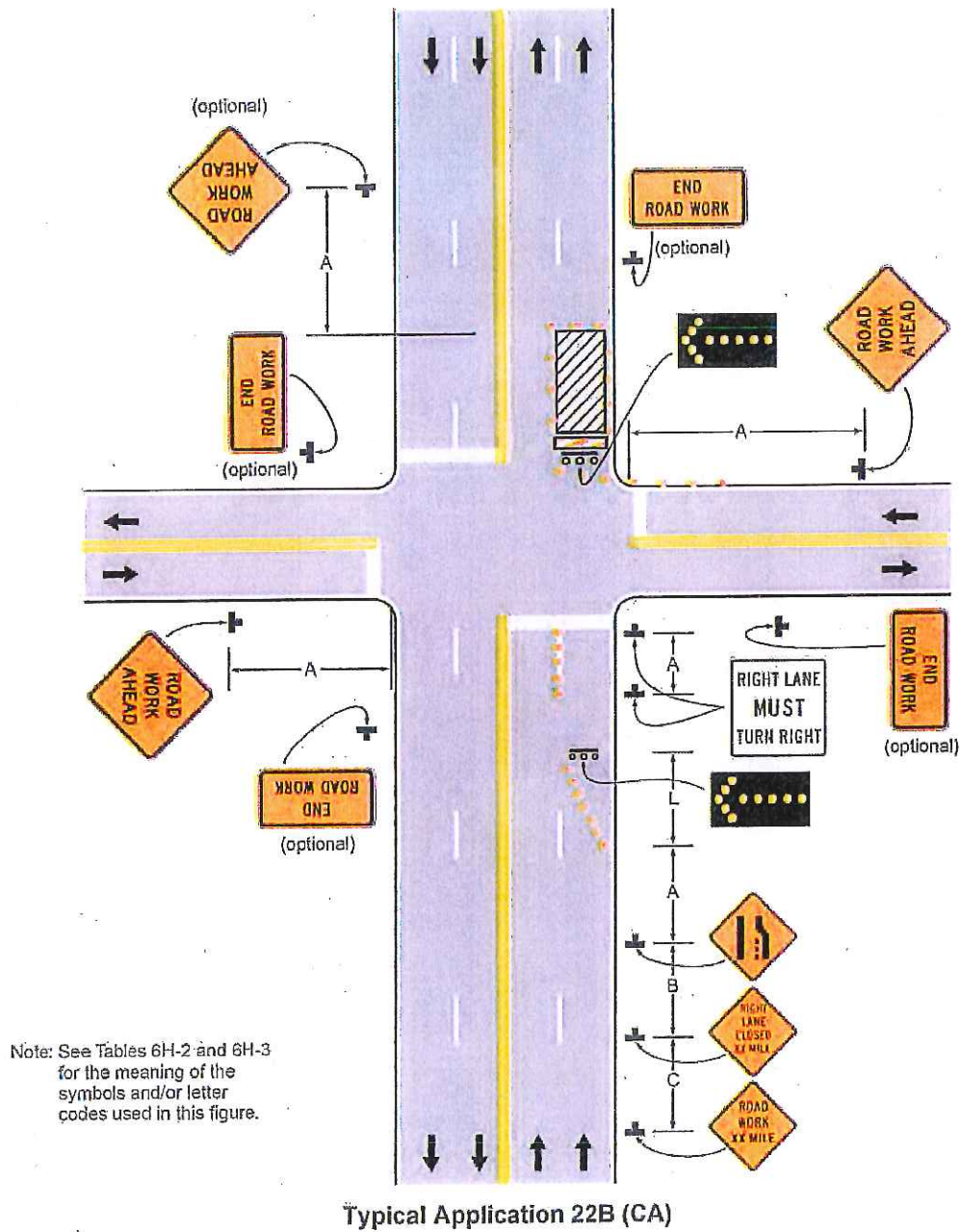
Figure 6H-22B(CA). Right-Hand Lane Closure on the Far Side of an Intersection (TA-22B (CA))
