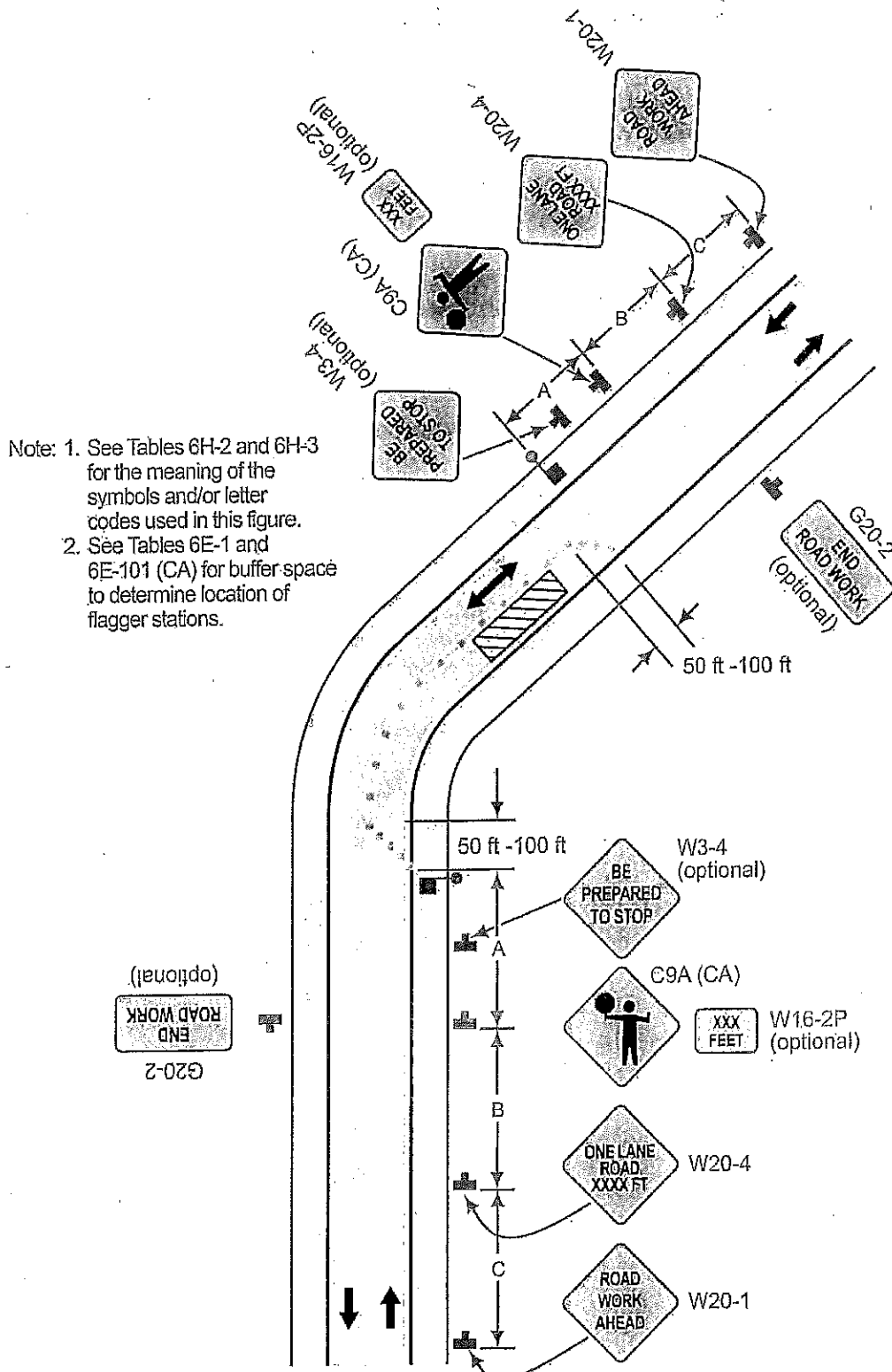
Typical Application 10
