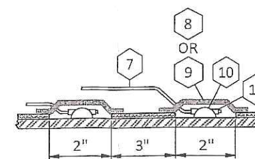
DETAIL 4 SCALE: NO SCALE ATTACHING THE WIRES TO THE GAS MAIN (CCV O-10) FIGURE 1
