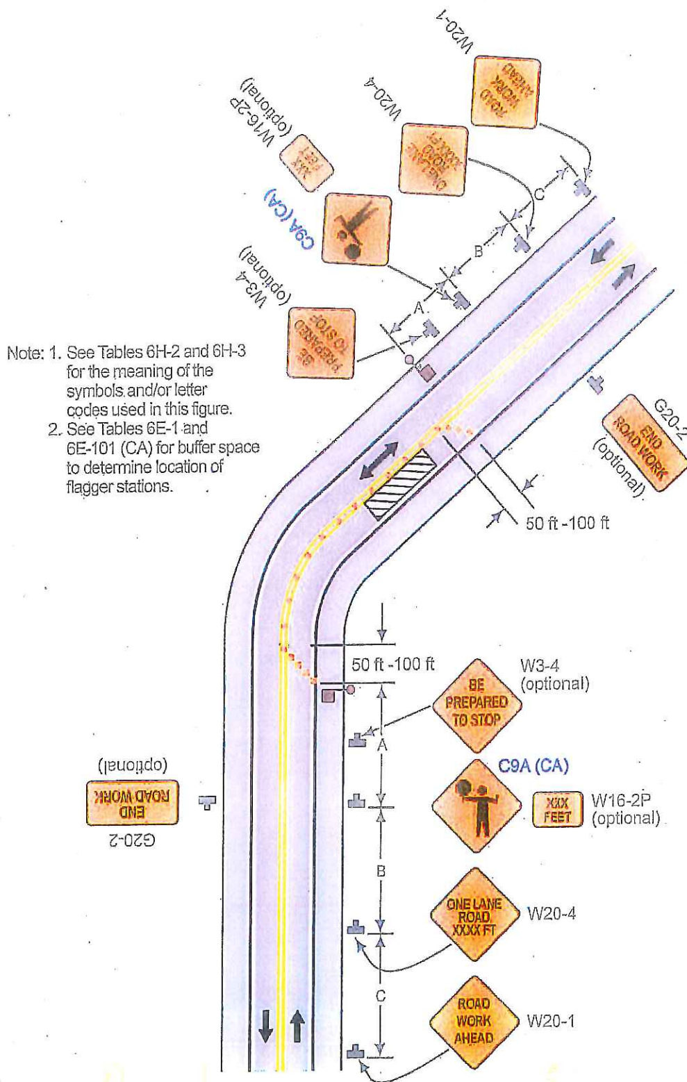
Typical Application 10
