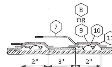
DETAIL 4 ATTACHING THE WIRES TO THE GAS MAIN (CCV O-10) FIGURE 1 SCALE: NO SCALE
