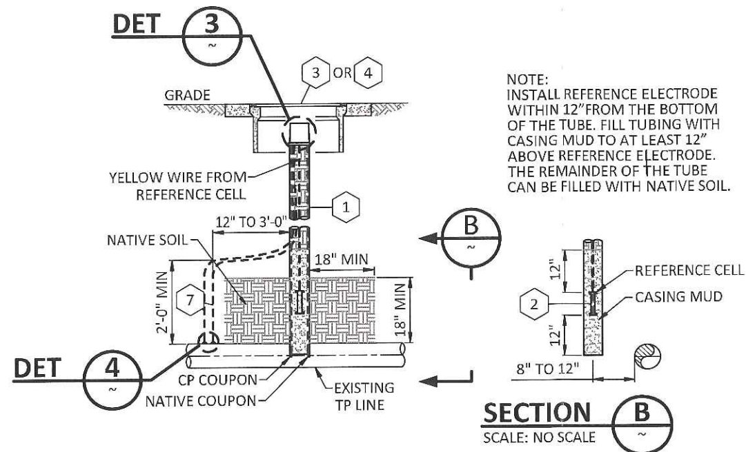
DETAIL 2 SCALE: NO SCALE SHTS 7-23 COUPON TEST STATION BELOW GROUND CCV O-10.2
