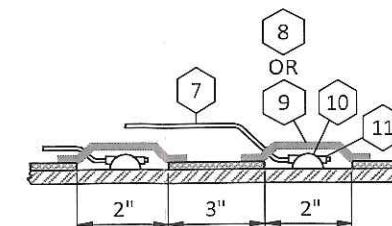
DETAIL 4 SCALE: NO SCALE ATTACHING THE WIRES TO THE GAS MAIN (CCV O-10) FIGURE 1
