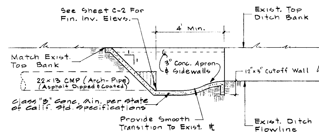
PIPE ENTRANCE DETAIL Scale: 3/8" = 1'-0"
