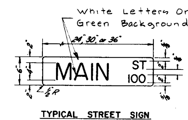
TYPICAL STREET SIGN
