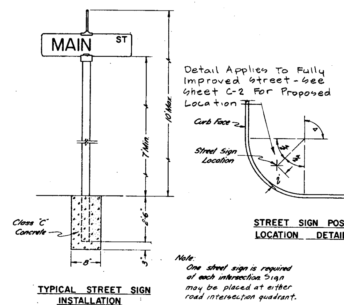
STANDARD STREET SIGN DETAILS
