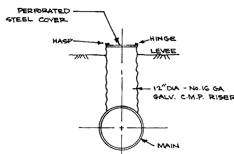
RISER FOR SIPHON BREAKER nts
