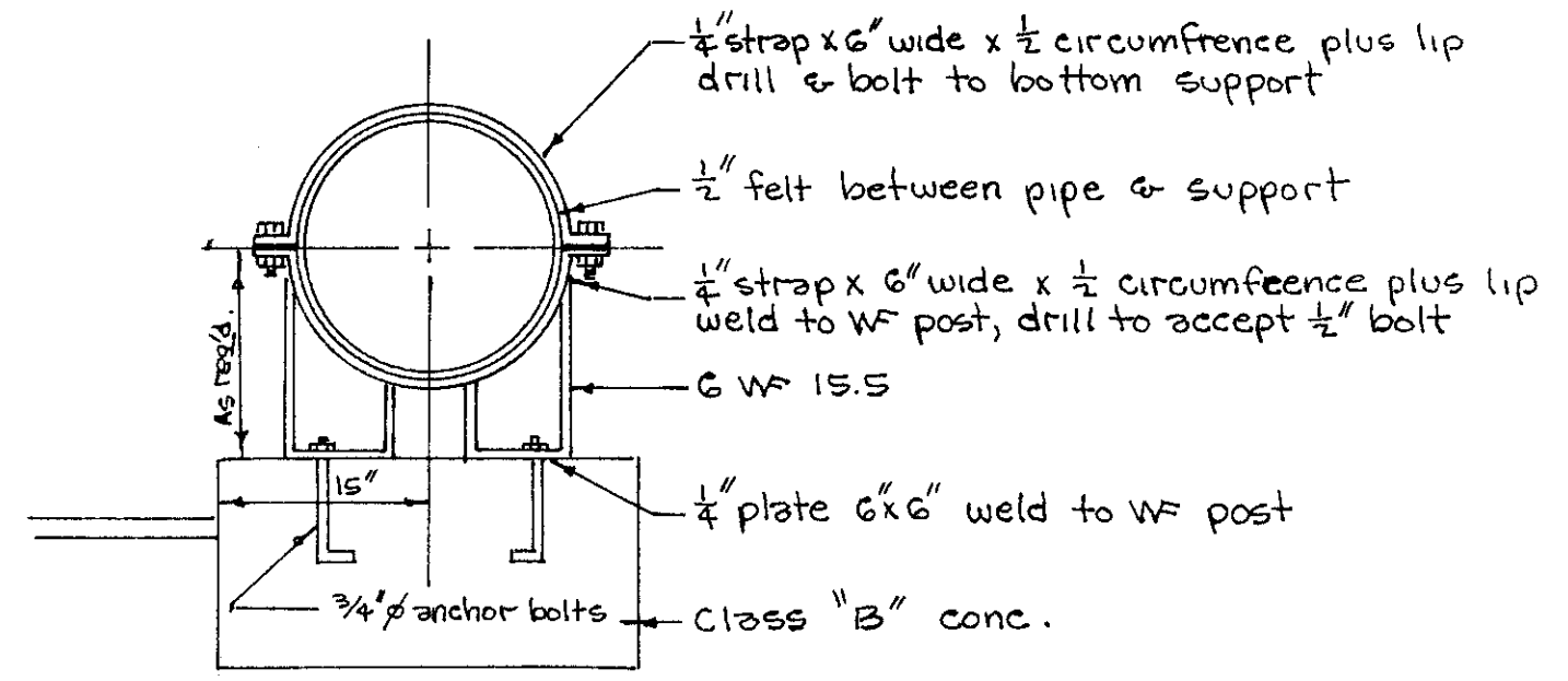
PIPE SUPPORT
