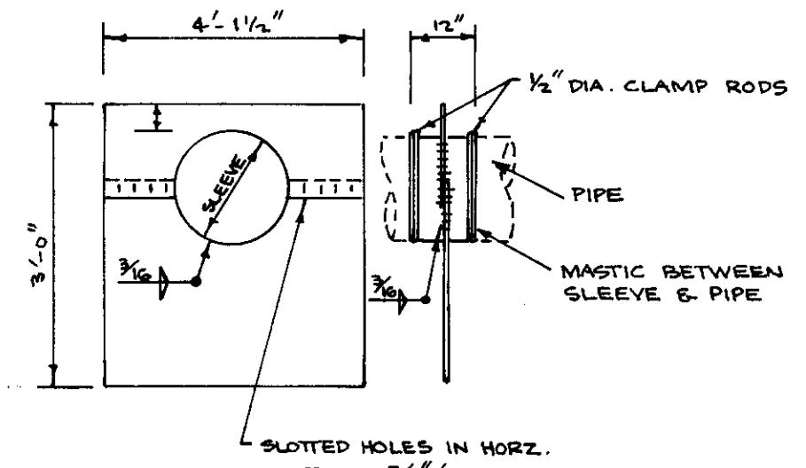
PLATE STEEL CUT-OFF WALL nts
