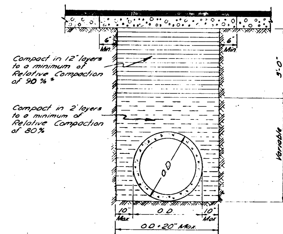
TYPICAL TRENCH BACKFILL DETAIL
