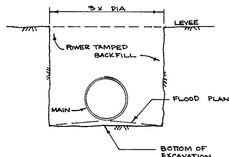
EXCAVATION & BACKFILL nts
