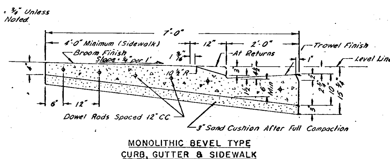
CURB, GUTTER & SIDEWALK SUBDIVISION STREETS
