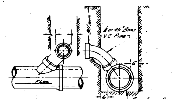
TYPICAL "Y" JOINT SERVICE CONNECTION
