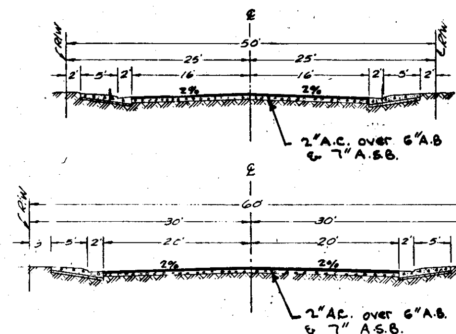
TYPICAL SUBDIVISION STREETS
