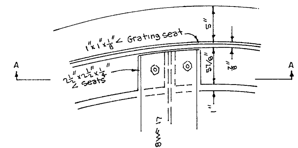
BEAM SEAT DETAIL
