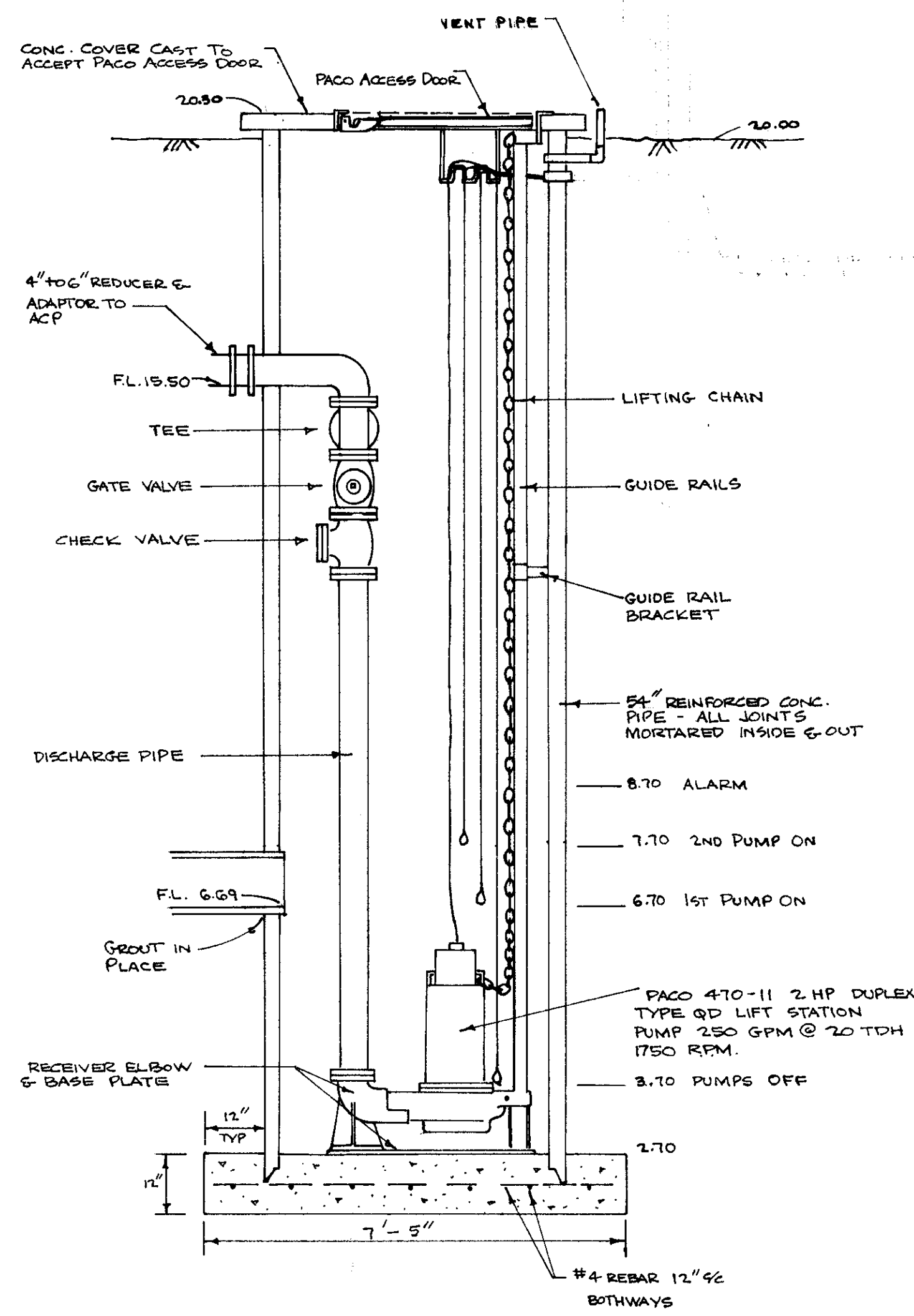
DETAIL 1/2" = 1'-0"
