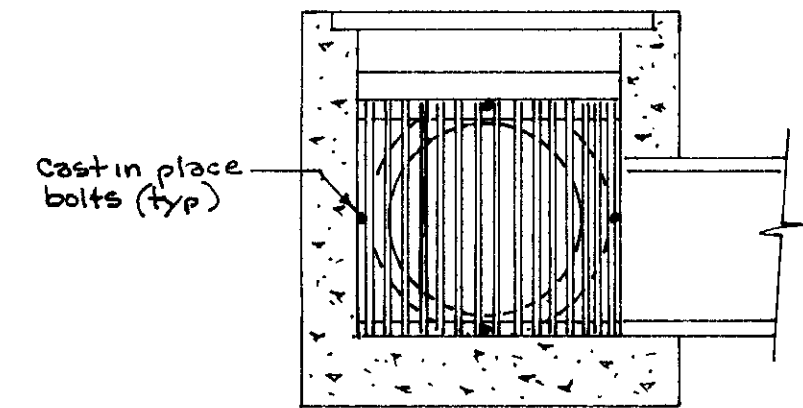
TRASH RACK DETAIL
