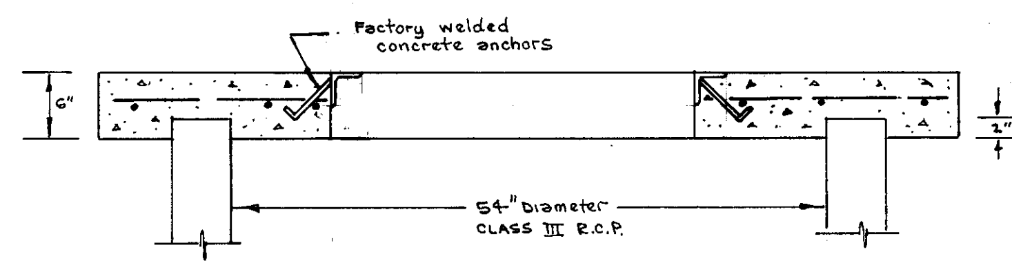
LIFT STATION COVER DETAIL SCALE 1" = 1'-0"
