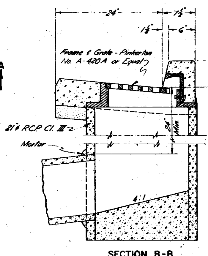
SECTION B-B
