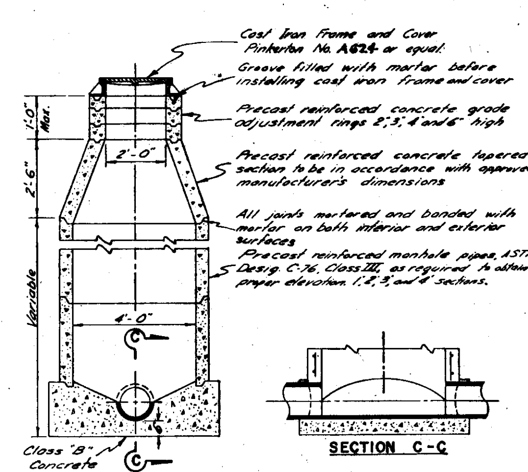
TYPICAL SANITARY SEWER MANHOLE
