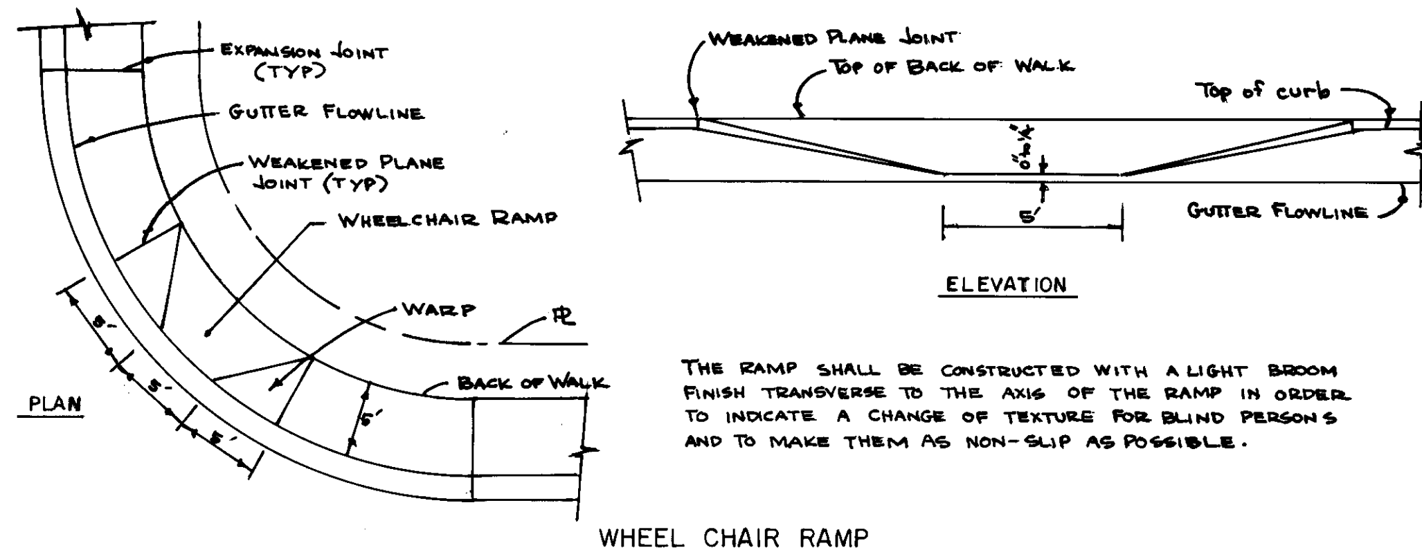
WHEEL CHAIR RAMP
