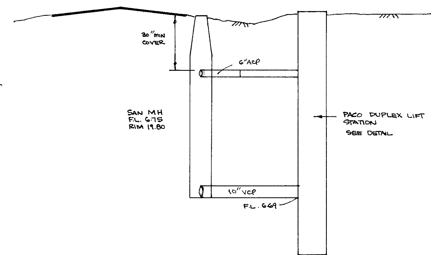
SECTION
