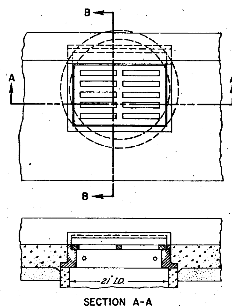
STANDARD STORM DRAIN INLET
