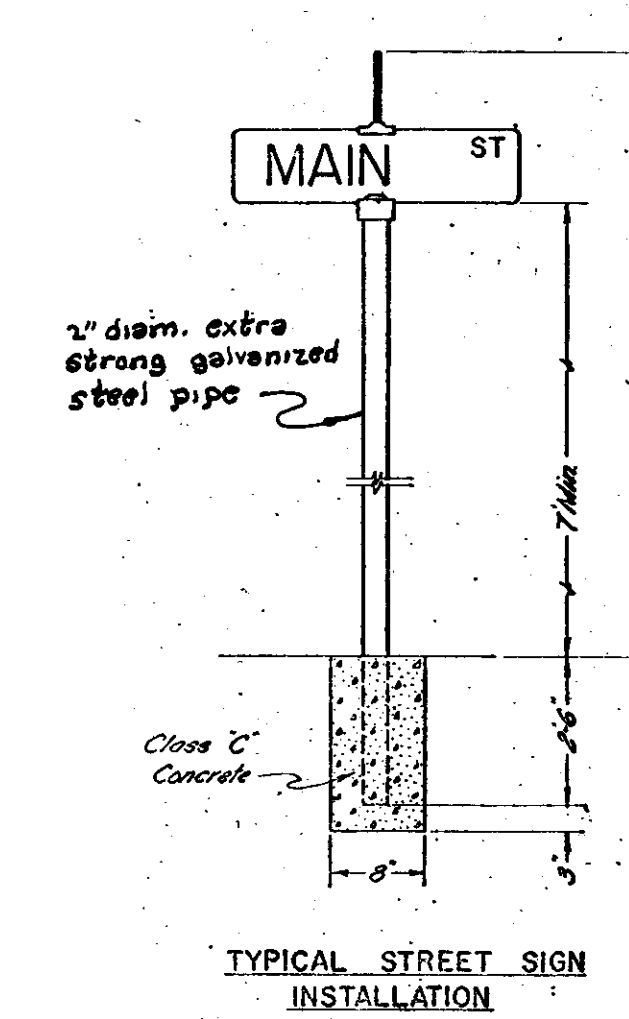
STANDARD STREET SIGN DETAILS
