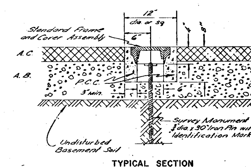
TYPICAL SECTION
