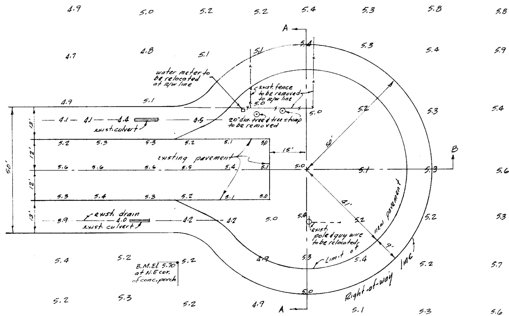
SONORA STREET - PLAN - (showing existing features) scale: 1"=20'
