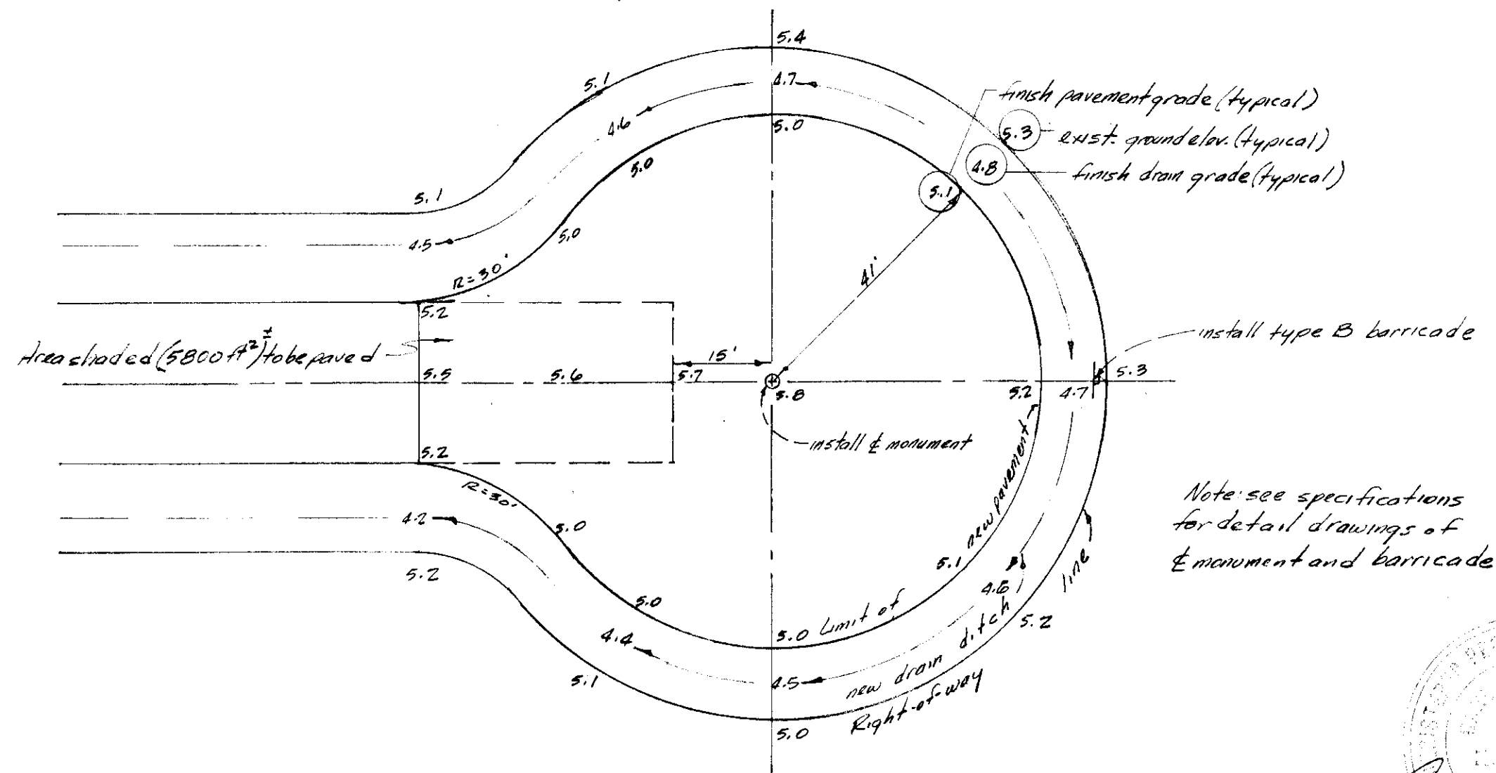
SONORA STREET - PLAN - (showing existing features) scale: 1"=20'
