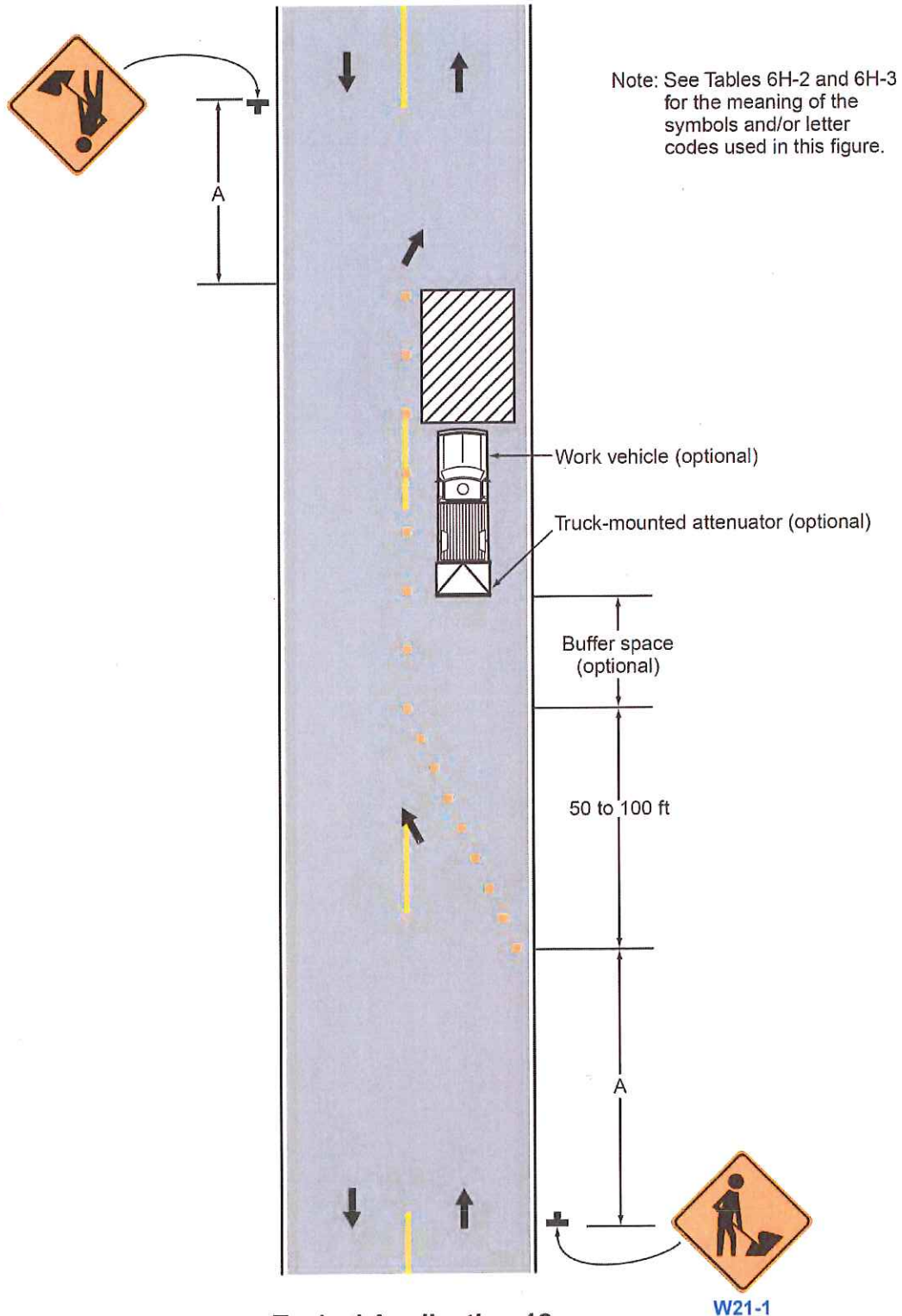
Typical Application 18
