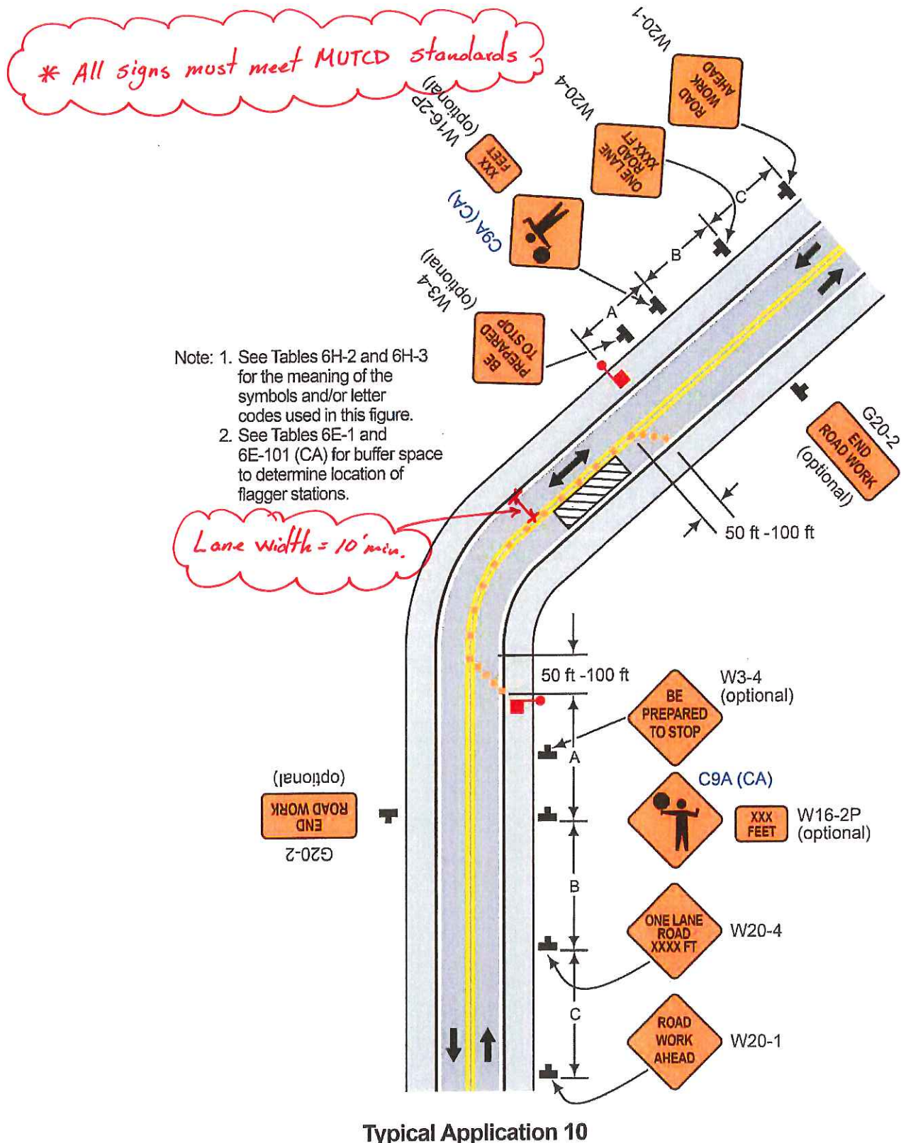
Figure 6H-10 (CA). Lane Closure on Two-Lane Road Using Flaggers (TA-10)
