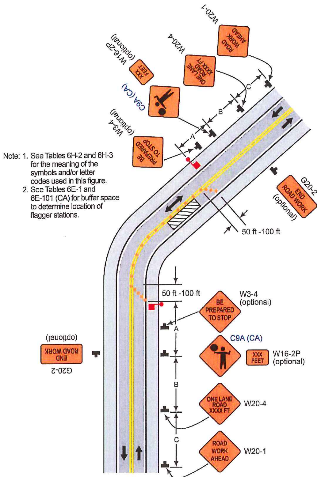
Typical Application 10
