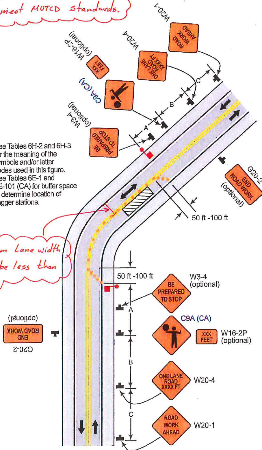
Typical Application 10
