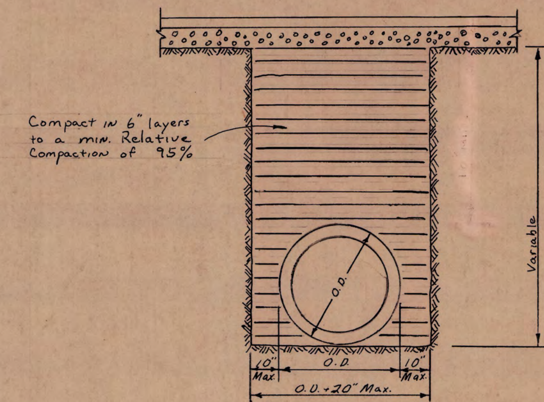
TYPICAL TRENCH BACKFILL DETAIL
