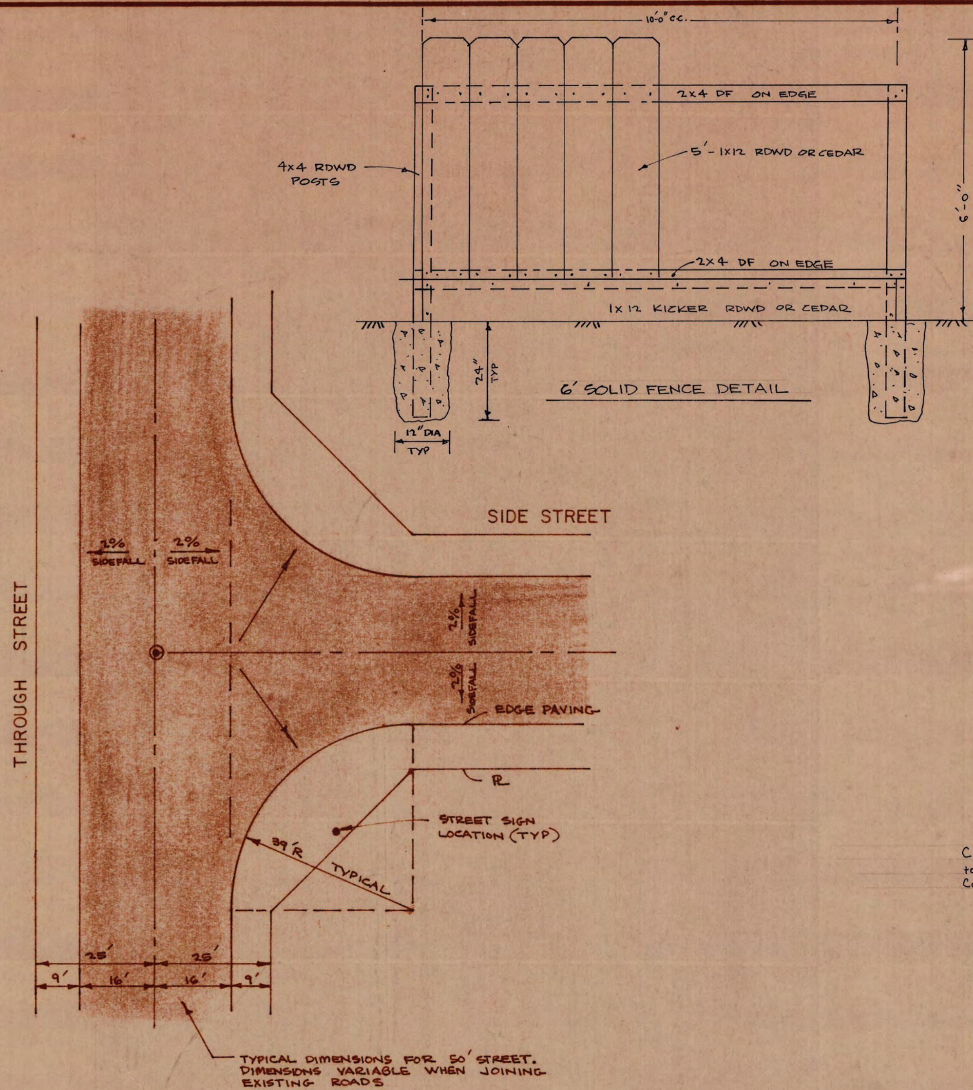
TYPICAL TEE INTERSECTION DETAIL
