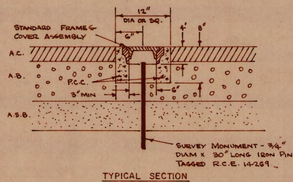
SURVEY MONUMENT FRAME & COVER ASSEMBLY
