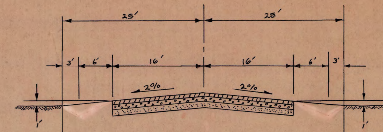
50' INTERIOR ROAD TYPICAL SECTION
