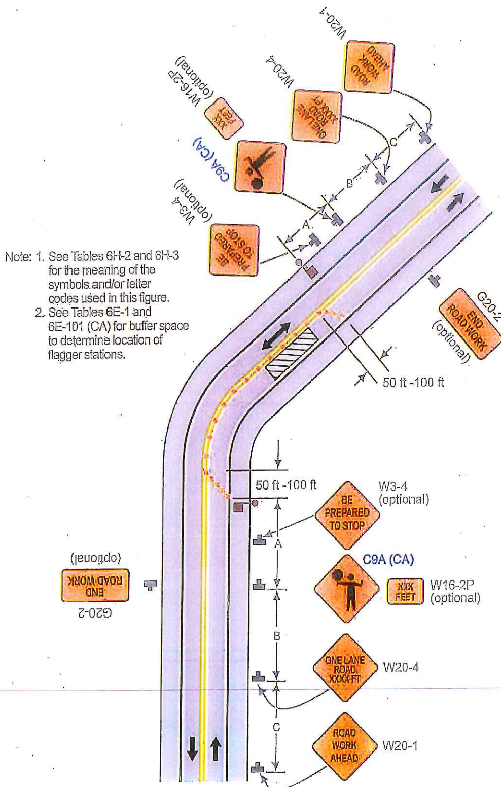
Typical Application 10
