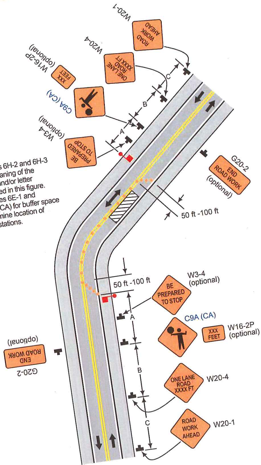
Typical Application 10
