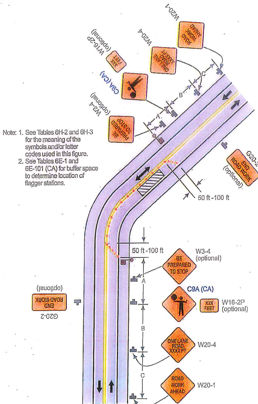
Typical Application 10
