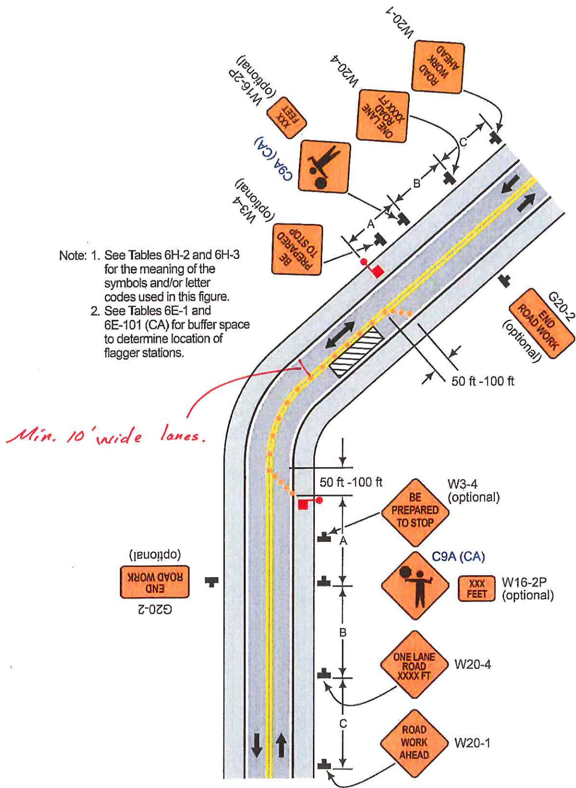
Typical Application 10
