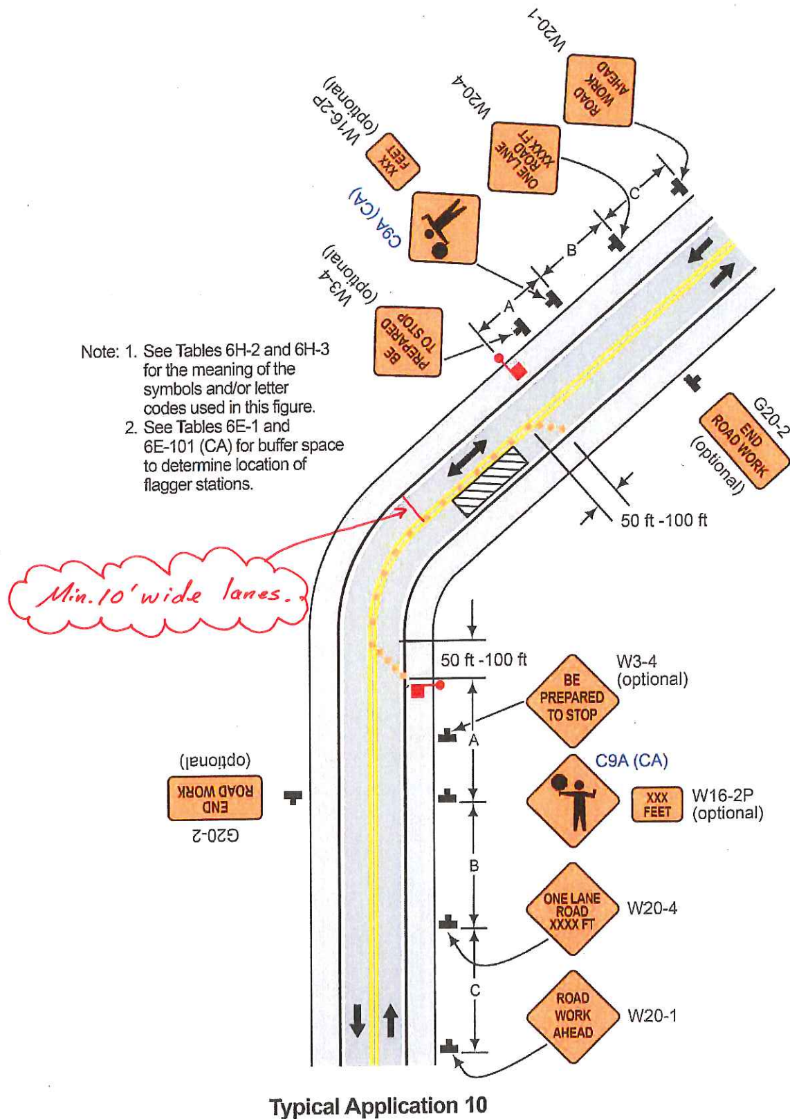
Figure 6H-10 (CA). Lane Closure on Two-Lane Road Using Flaggers (TA-10)
