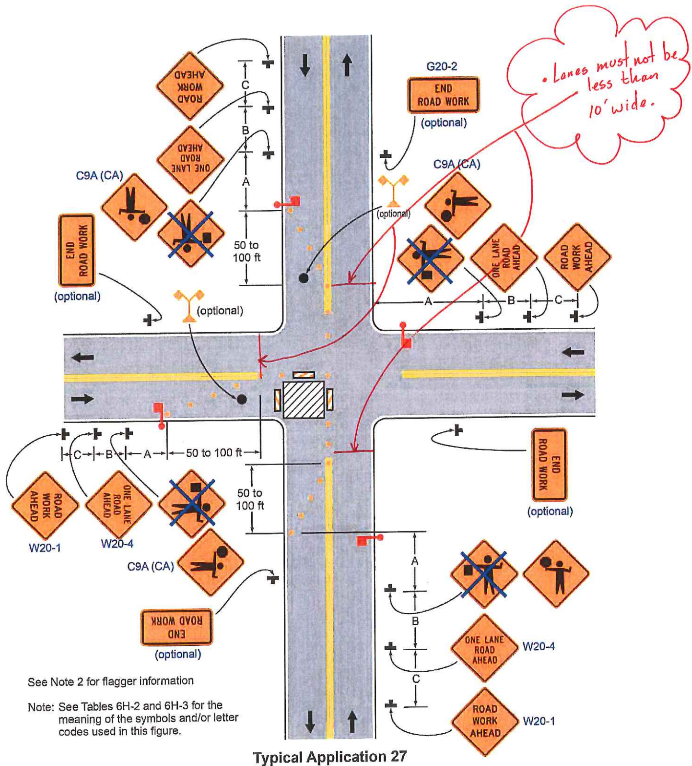
Figure 6H-27. Closure at the Side of an Intersection (TA-27)
