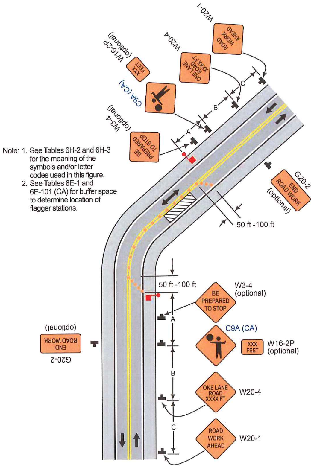
Typical Application 10
