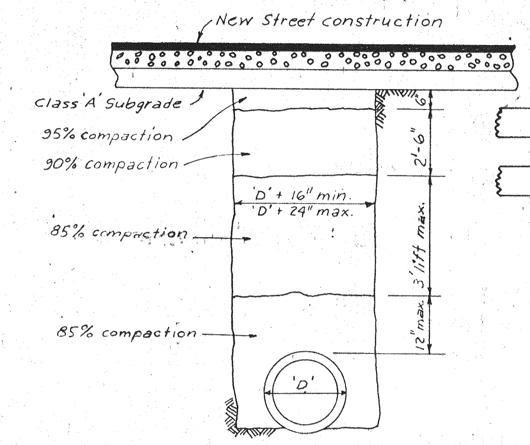
TYPICAL SECTION in New Street Construction and Unimproved Street right-of-way or Easements.
