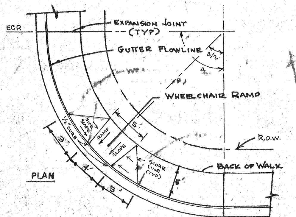
CURB, GUTTER & SIDEWALK SUBDIVISION STREETS
