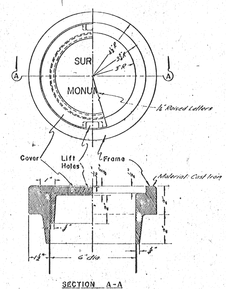
SURVEY MONUMENT FRAME AND COVER ASSEMBLY
