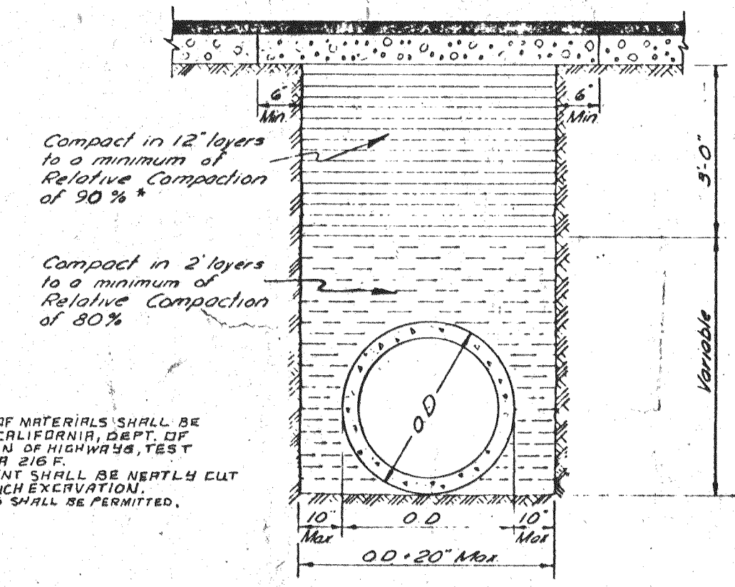
TYPICAL TRENCH BACKFILL DETAIL STORM DRAIN AND WATER
