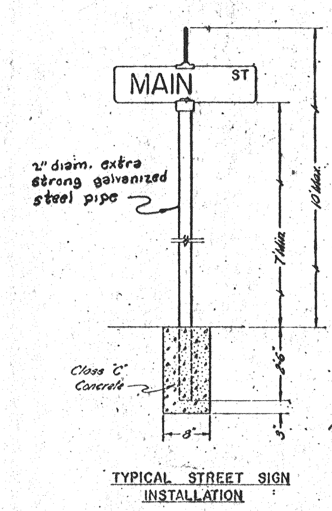
STANDARD STREET SIGN DETAILS
