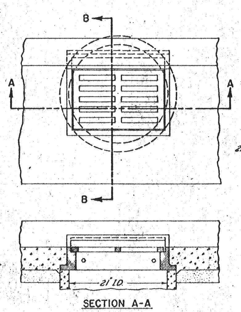
STANDARD STORM DRAIN INLET
