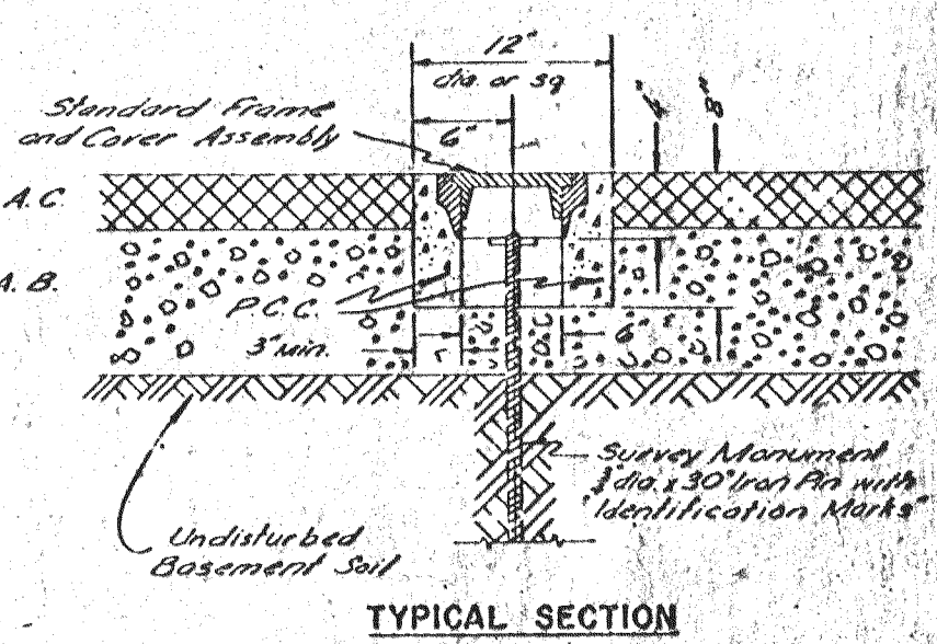
SURVEY MONUMENT FRAME AND COVER ASSEMBLY
