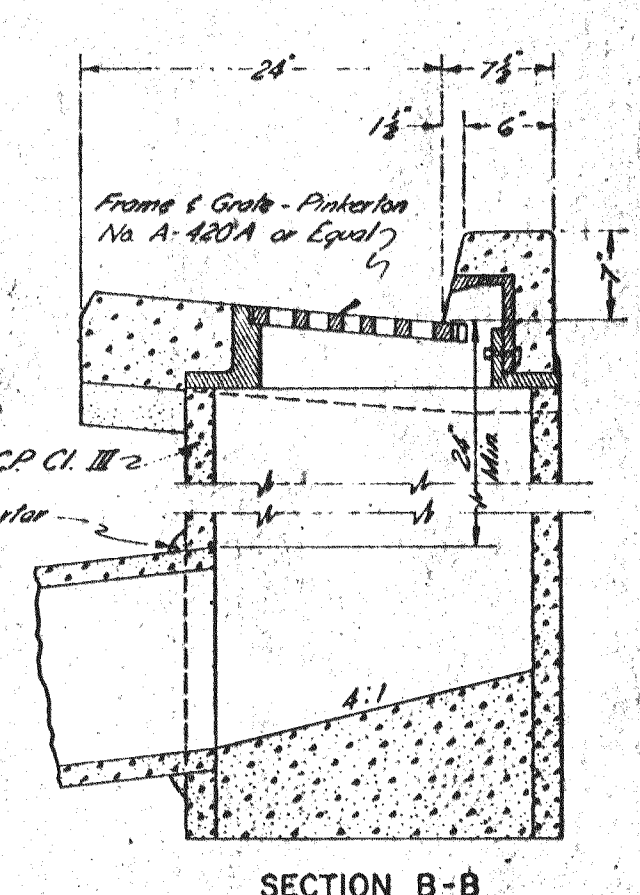
SECTION B-B
