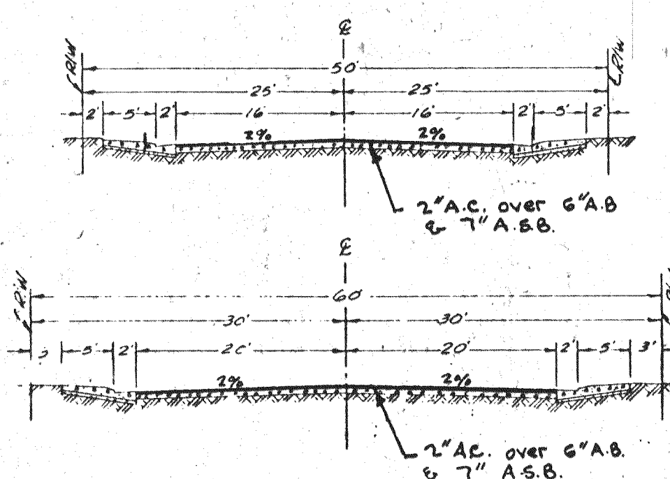
TYPICAL SUBDIVISION STREETS
