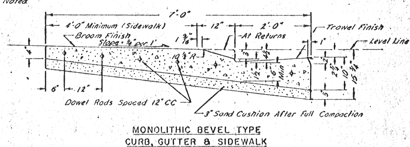
CURB, GUTTER & SIDEWALK SUBDIVISION STREETS
