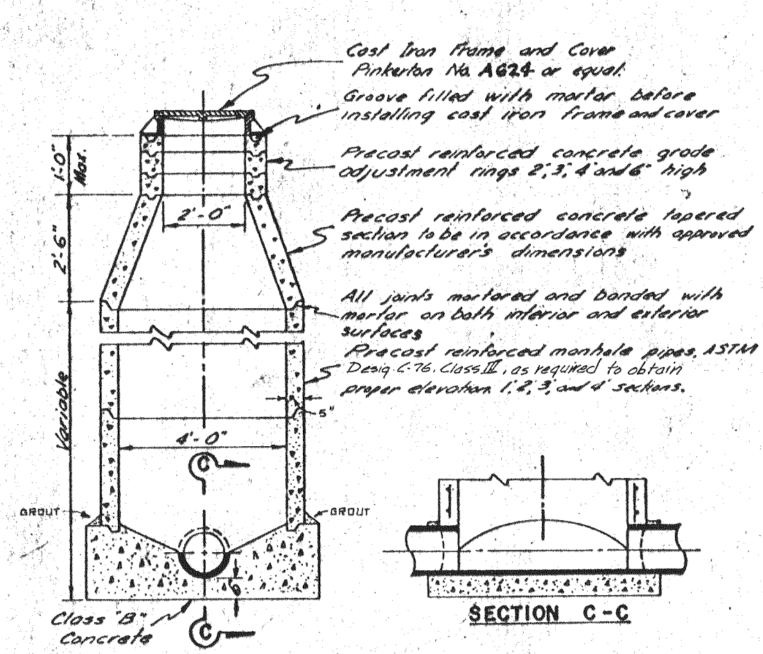
TYPICAL SANITARY SEWER MANHOLE
