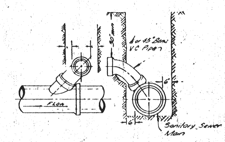
TYPICAL "Y" JOINT SERVICE CONNECTION
