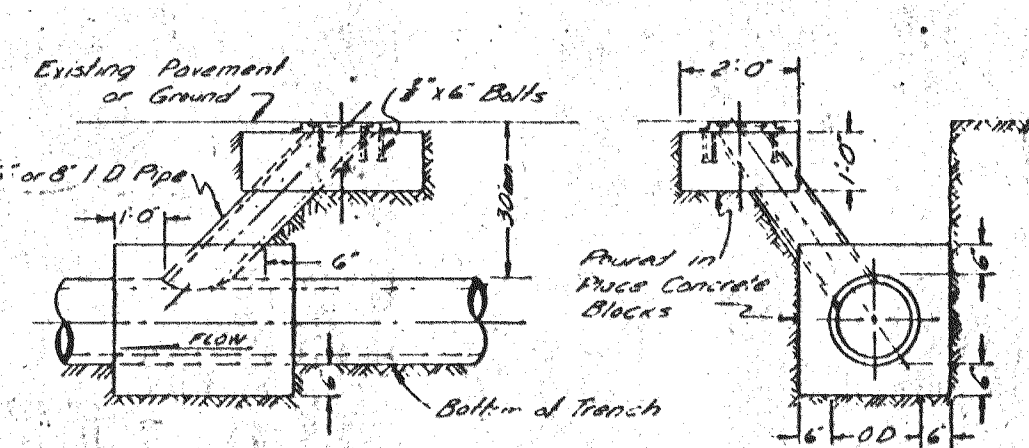
TYPICAL LAMPHOLE INSTALLATION
