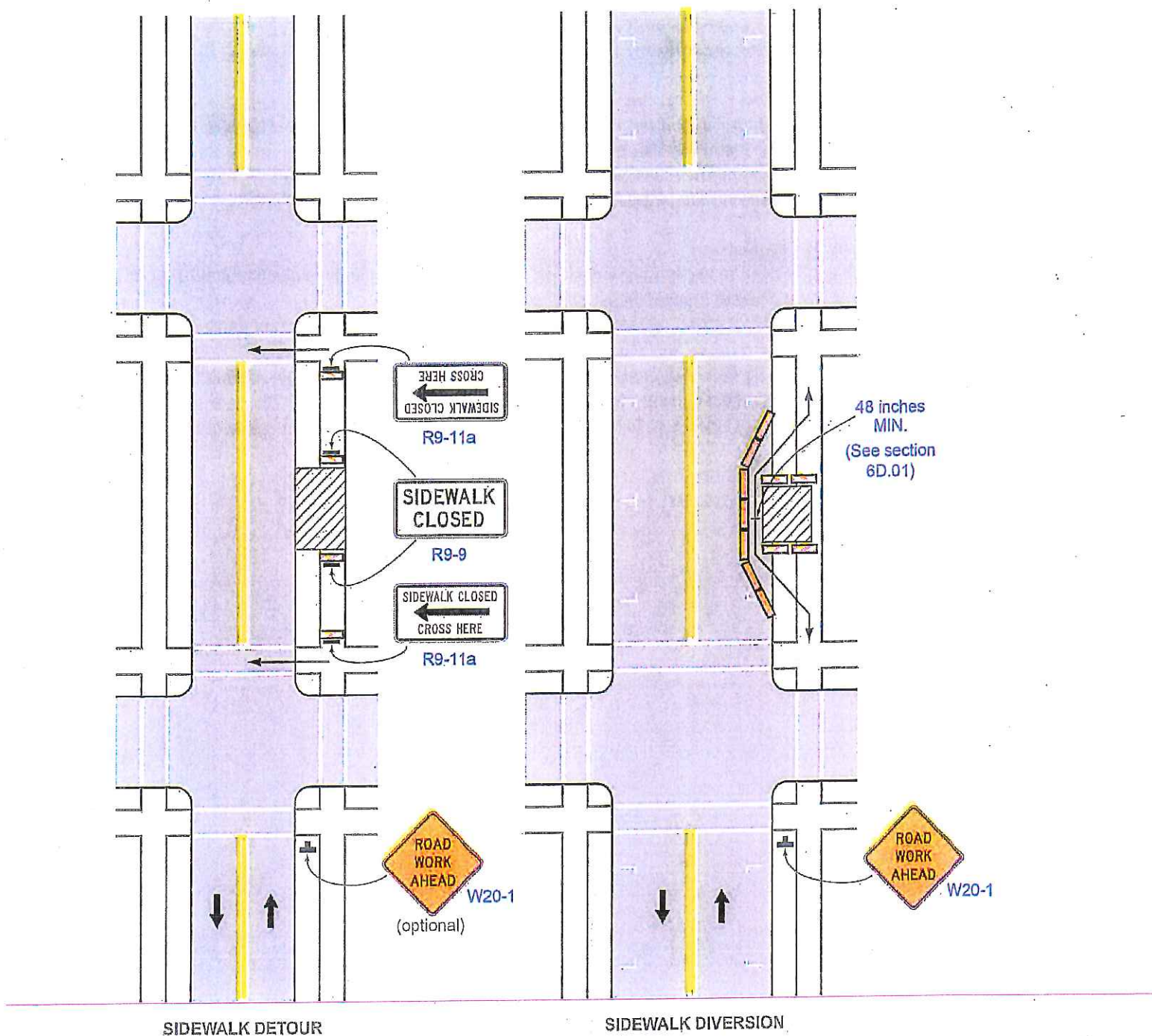
Figure 6H-28. Sidewalk Detour or Diversion (TA-28)
