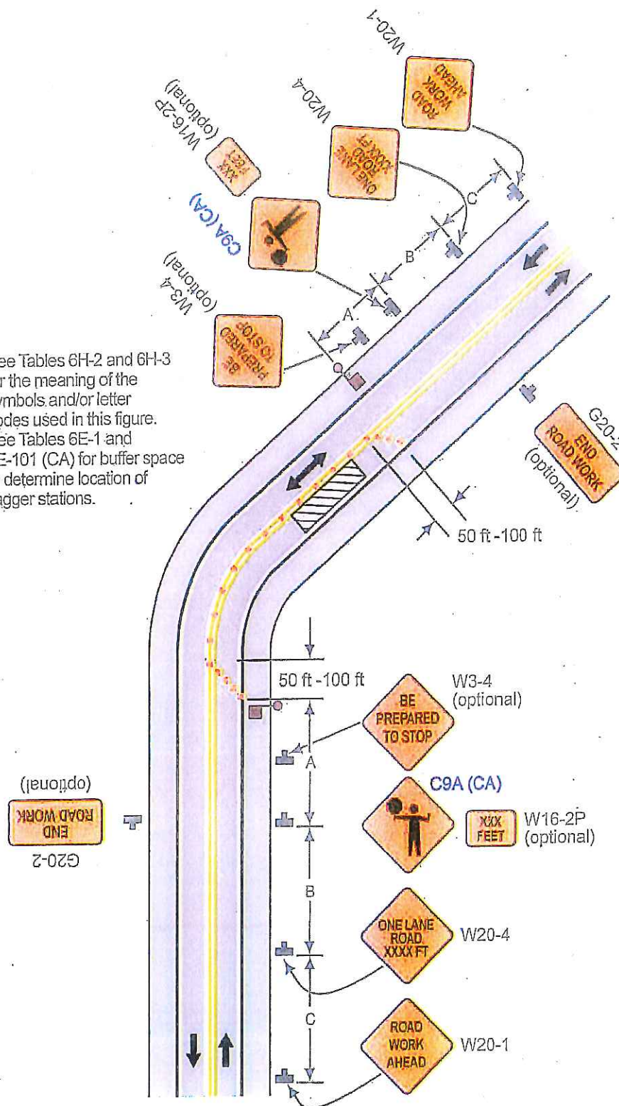
Typical Application 10
