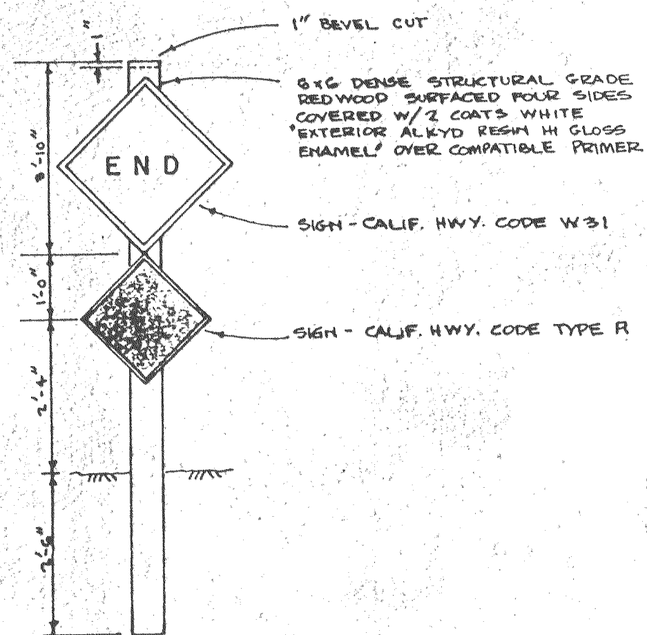
TYPE "B" BARRICADE
