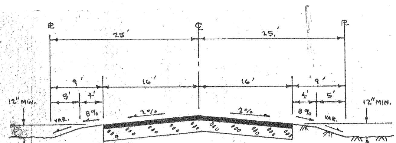
TYPICAL SECTION n.s.
