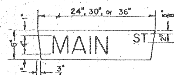
TYPICAL STREET SIGN
