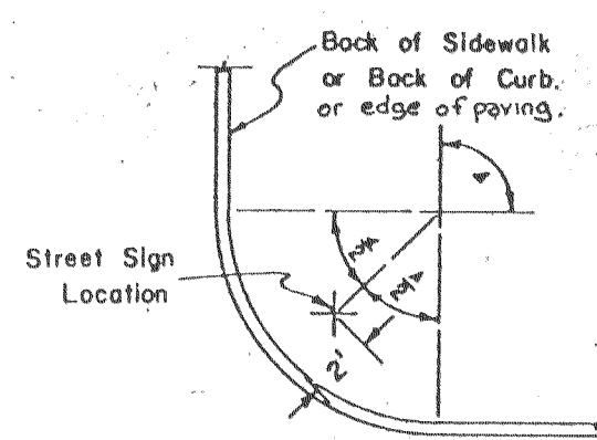
STREET SIGN POST LOCATION DETAIL
