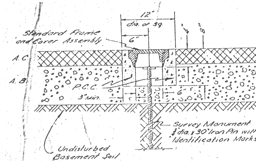
TYPICAL SECTION
