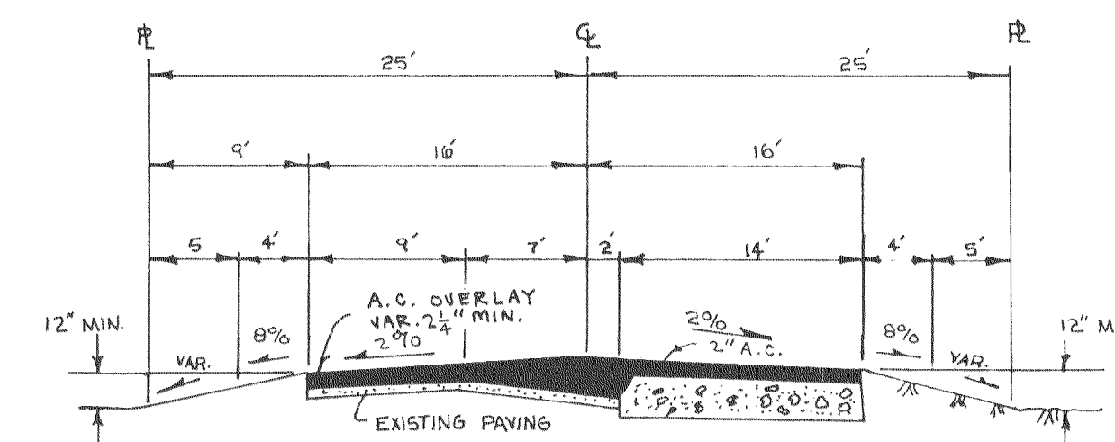
DILL COURT TYPICAL SECTION n.i.s.
