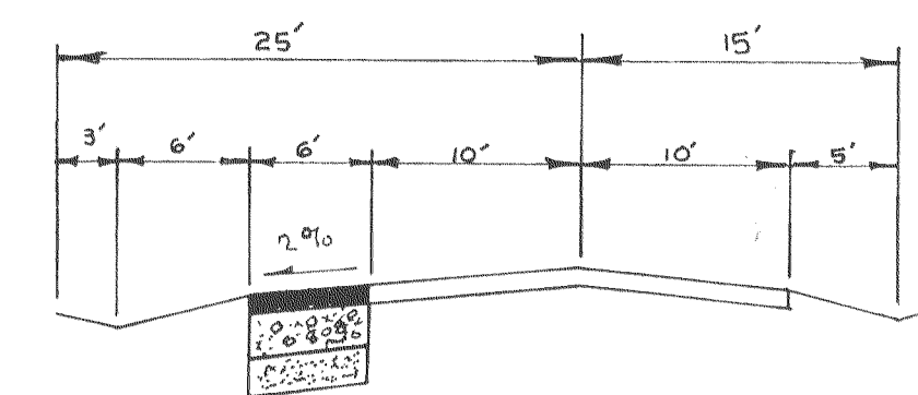
WHITE LANE TYPICAL SECTION n.i.s.
