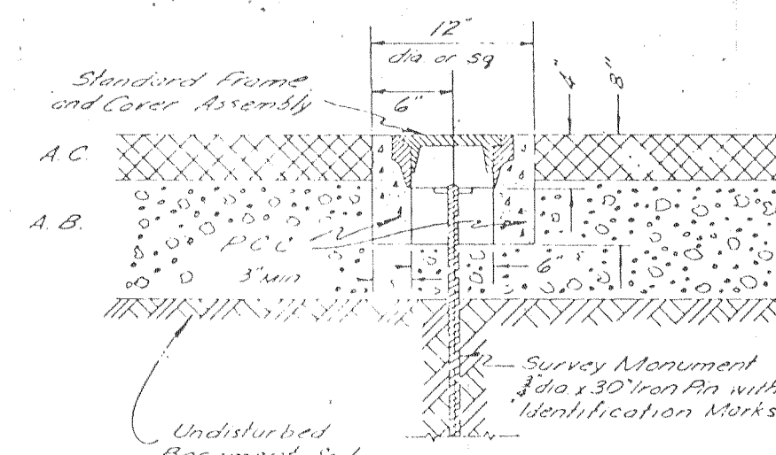
TYPICAL SECTION
