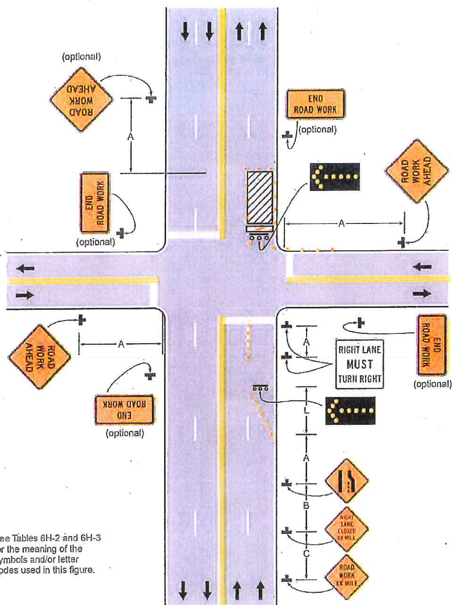
Typical Application 22B (CA)
