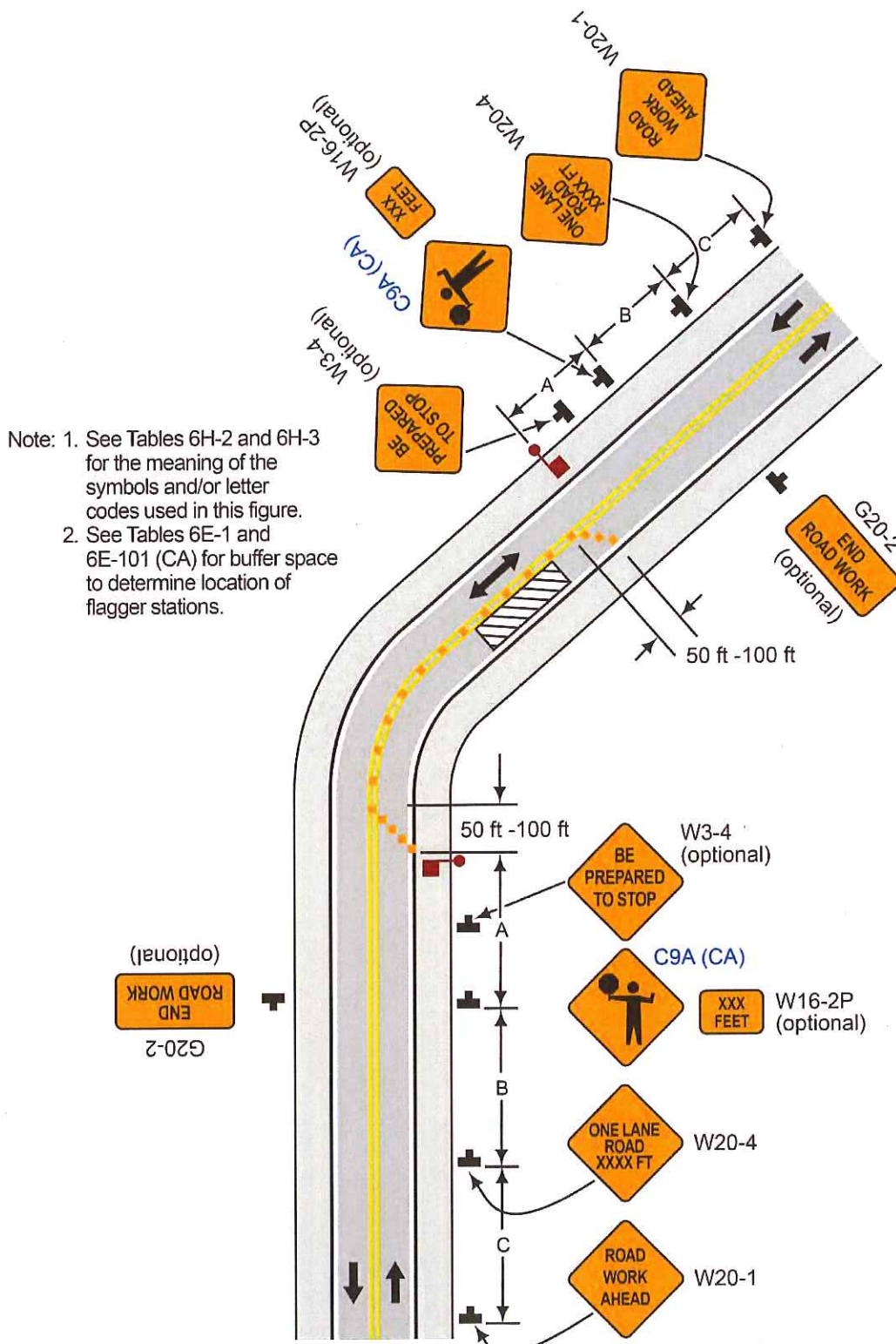
Typical Application 10
