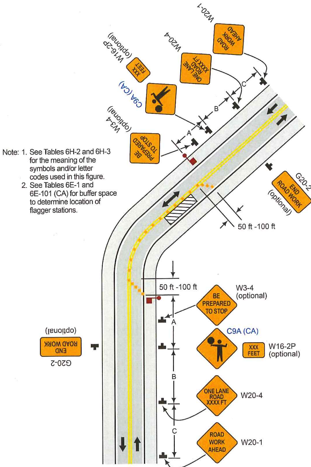
Typical Application 10
