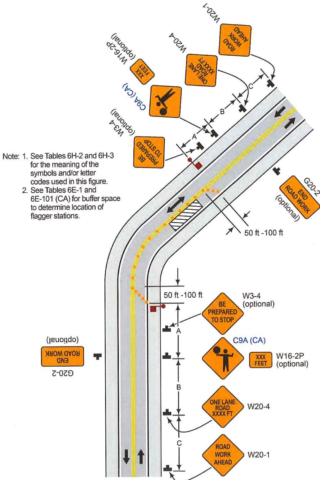
Typical Application 10
