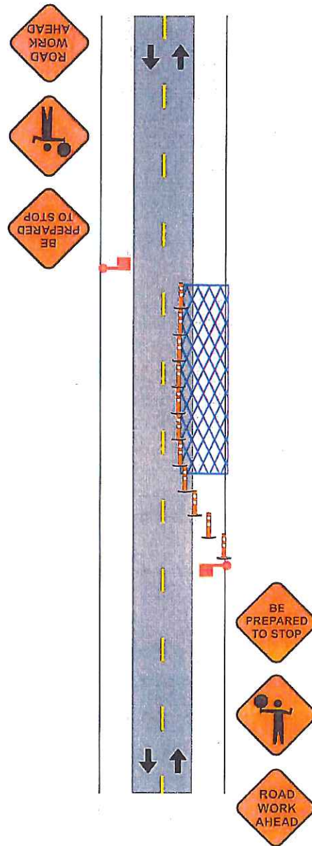
Typical Application 13
