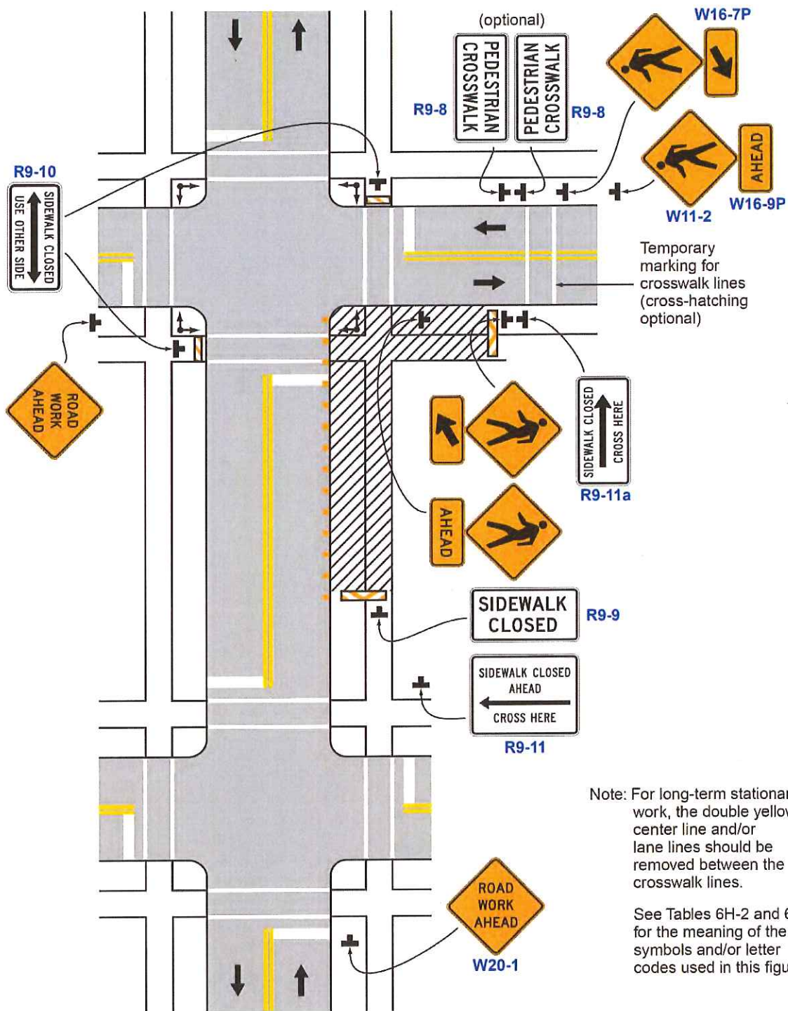
Typical Application 29
